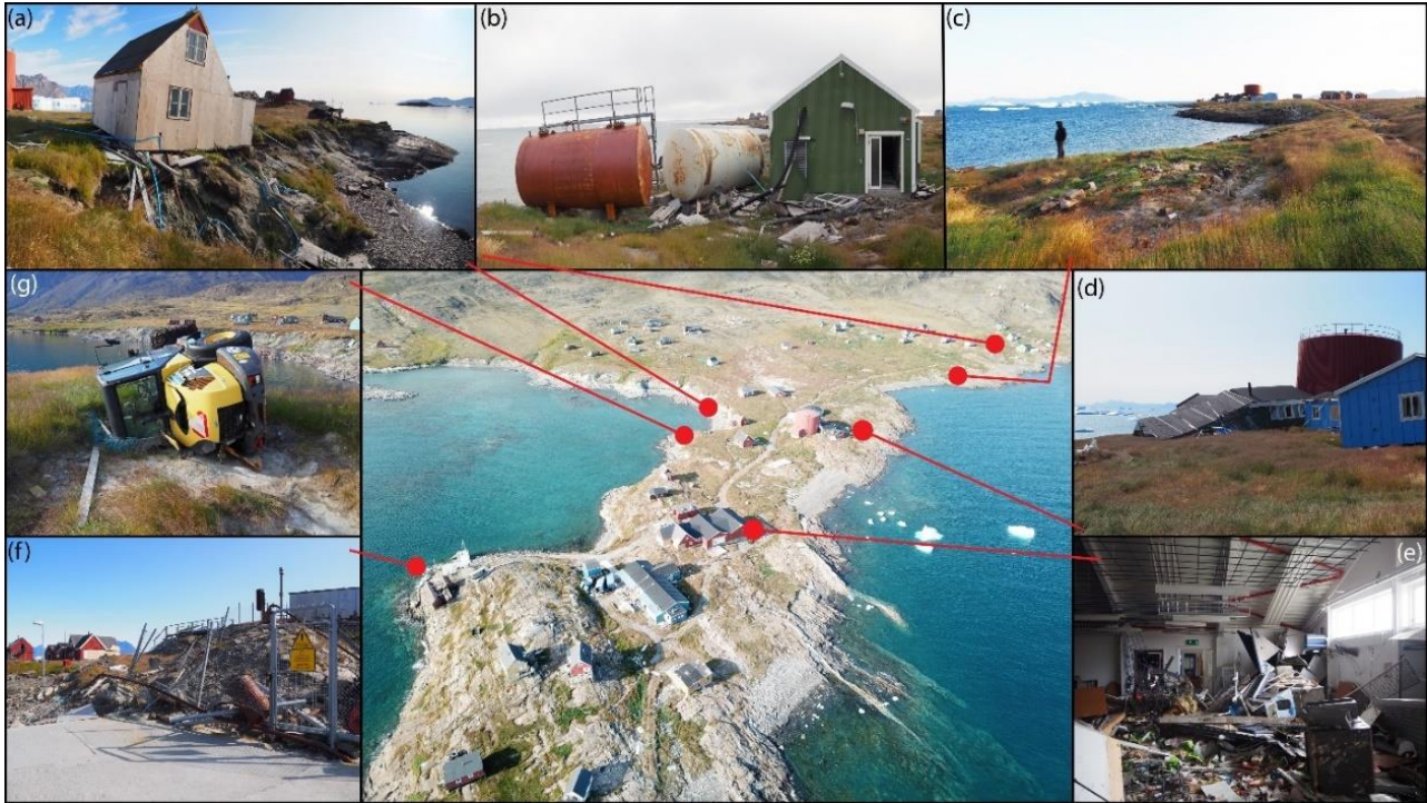
Figure 8. Examples of infrastructure damages caused by 2017 tsunami in Nuugaatsiaq. (a) Wooden house removed by wave from point foundation transported several dozen of meters; (b) Fuel tanks washed away from concrete frames and pushed towards power plant. Note large accumulation of litter and tsunami deposits around and inside the buildings; (c) site of former building position, which was destroyed and swept away by tsunami. Note broken wooden point foundations, media connections and erosional gullies; (d) Smashed and collapsed wooden school building moved towards major water tank; (e) Interior of local shopping centre passed by tsunami. Note large amounts of litter and rotting food supplies and twisted and bowed metal frame construction; (f) Partly-torn metal fence around fuel storage site which acted as a trap for litter transported by tsunami; (g) example of heavy machine knocked over by waves.
