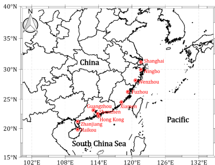
Figure 15: Locations of 10 selected coastal cities in China
