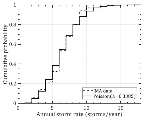
565 Figure 3: CDF of annual storm rate
