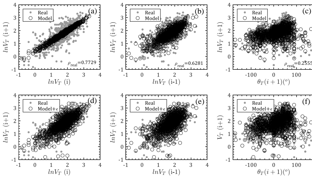
Figure 6: Comparison of translation speed between model and real observations: (a-c) relations between \ln V_T(i) , \ln V_T(i-1) , \theta(i+1) and \ln V_T(i+1) without errors; (d-f) relations between \ln V_T(i) , \ln V_T(i-1) , \theta(i+1) and \ln V_T(i+1) with errors; ( \rho_{real} is the correlation coefficient for real observation data)
