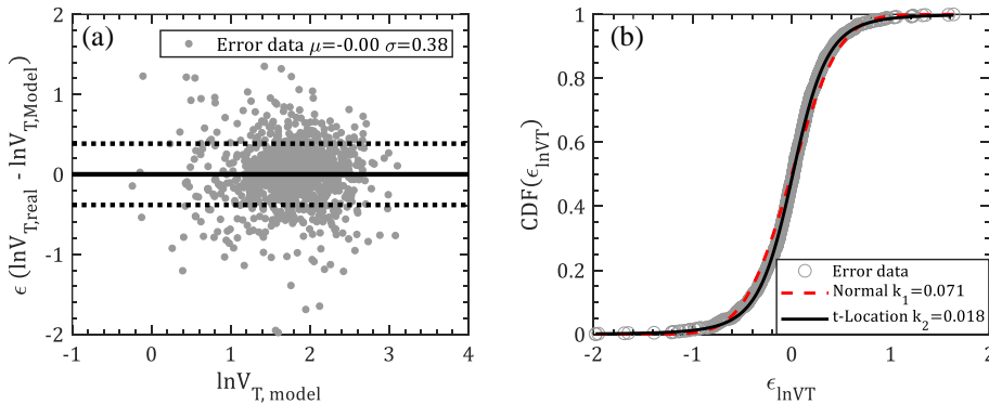
Figure 5: Logarithmic modelling errors for translation speed: (a) scatter plot; (b) CDF
