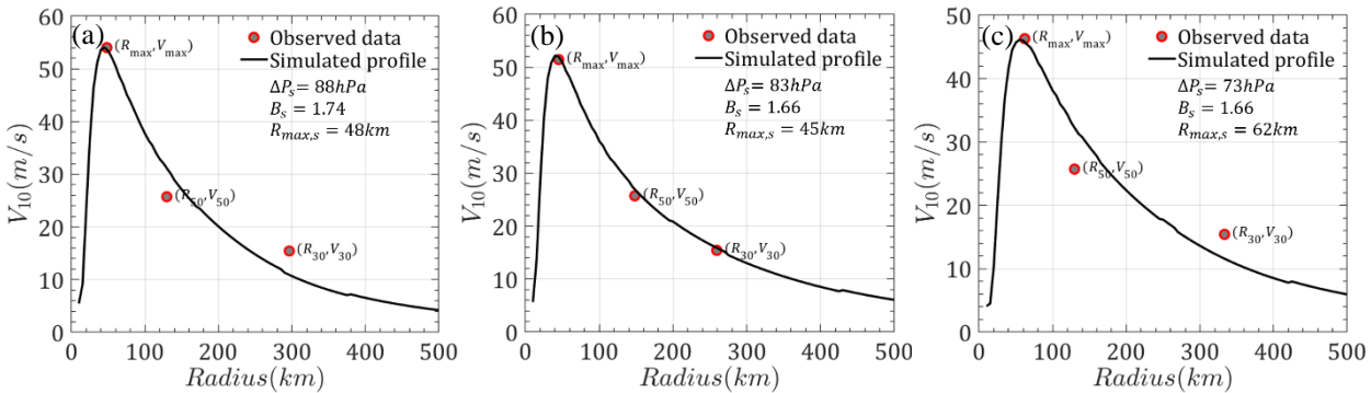
575 Figure 7: Radial wind speed profiles (a) Saomai (2006-08-09, 15:00UTC); (b) Parma (2009-10-01, 06:00UTC); (c) Rammason (2014-07-18, 12:00UTC)
