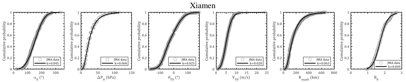
610 Figure 16: Empirical and preferable cumulative probability distributions for \alpha_0 , \Delta P_0 , \theta_0 , V_{T0} , R_{max,s0} and B_{s0}
