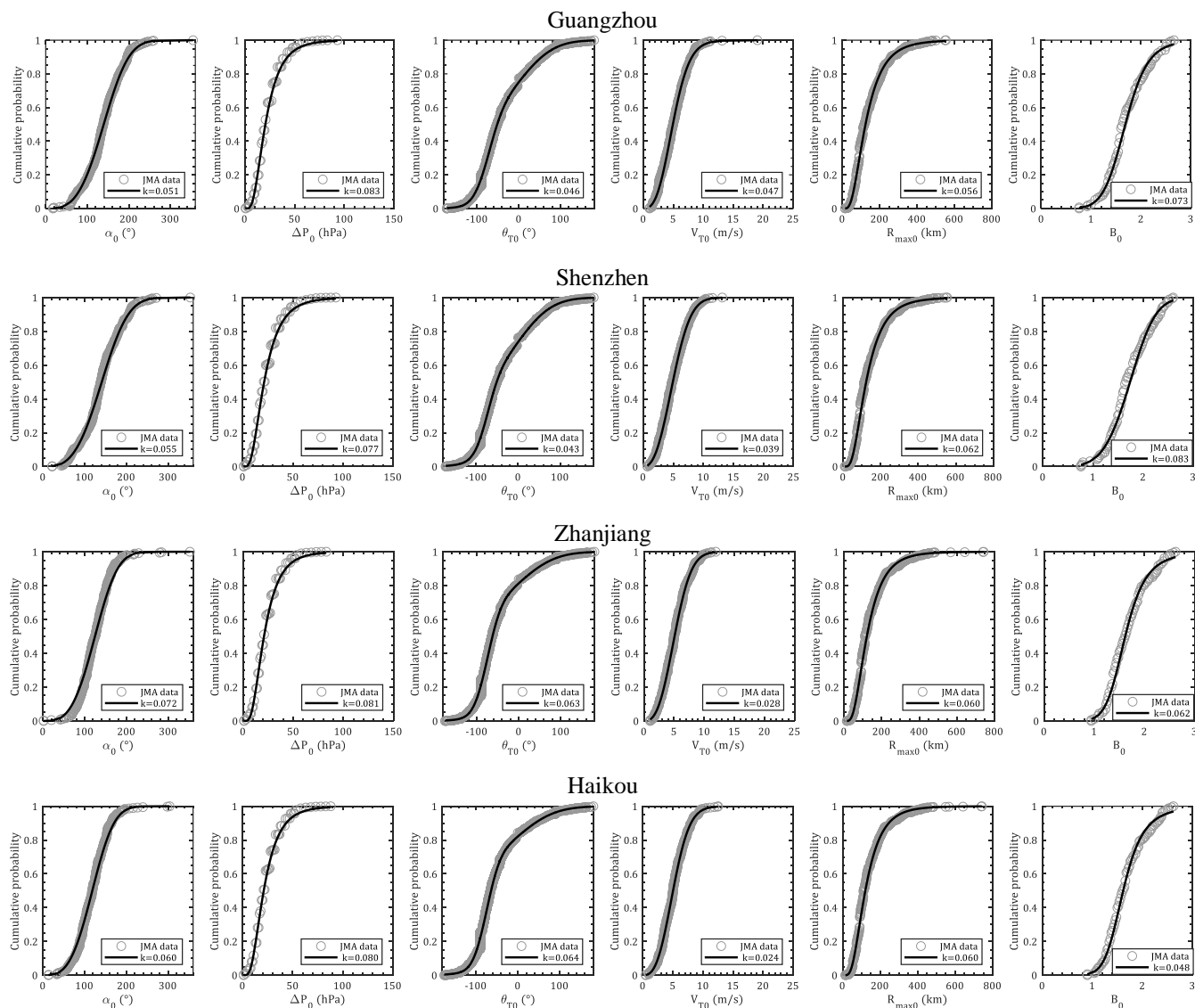
620 Figure 16 (Cont.): Empirical and preferable cumulative probability distributions for \alpha_0 , \Delta P_0 , \theta_0 , V_{T0} , R_{max,s0} and B_{s0}
