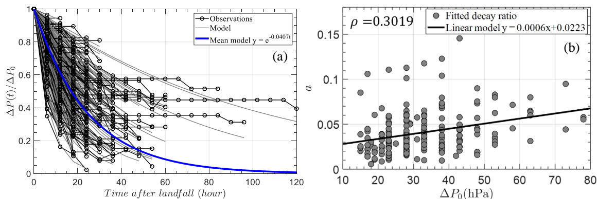
590 Figure 12: Decay model in circular sub-region around Hong Kong:(a) Curve fitting of decay model; (b) Decay rate versus \Delta P_0
