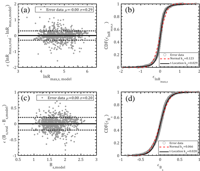
580 Figure 9: Model errors for \ln R_{max,s} and B_s : (a) scatter plot ( \epsilon_{\ln R_{max,s}} ); (b) CDF ( \epsilon_{\ln R_{max,s}} ); (c) scatter plot ( \epsilon_{B_s} ); (d) CDF ( \epsilon_{B_s} );
