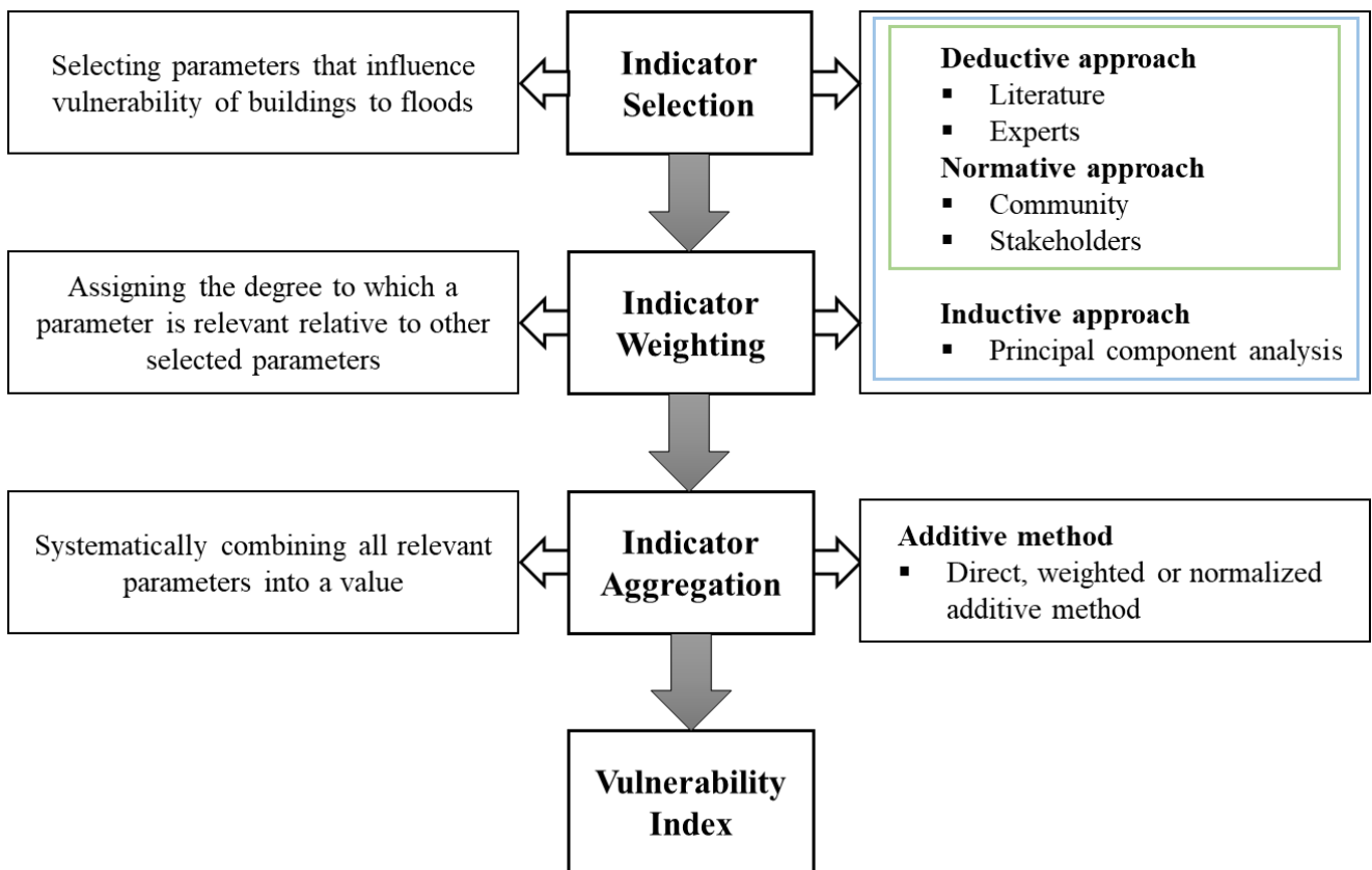
975 Figure 1: Steps and commonly applied methods for developing a physical flood vulnerability index. Steps include the indicator selection, the indicator weighting, and the indicator aggregation. Green box (applied for initial indicator selection) and blue box (applied for final indicator selection)
