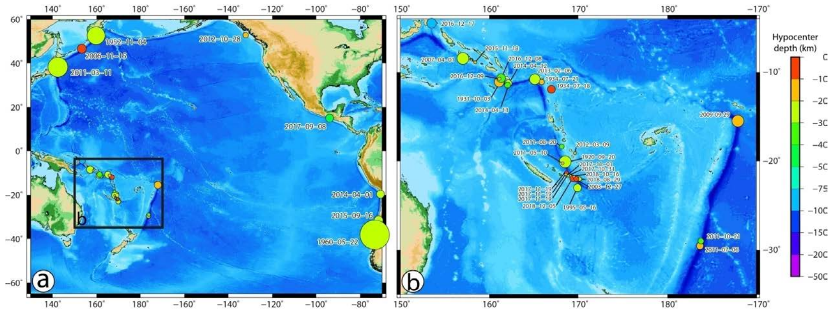
Figure 12 : Location of the epicenter of earthquakes having triggered tsunamis able to be reported or /recorded in New Caledonia. a) Over the whole Pacific Ocean highlighting source locations of transoceanic tsunamis ; b) at a regional scale, highlighting regional and local sources.
