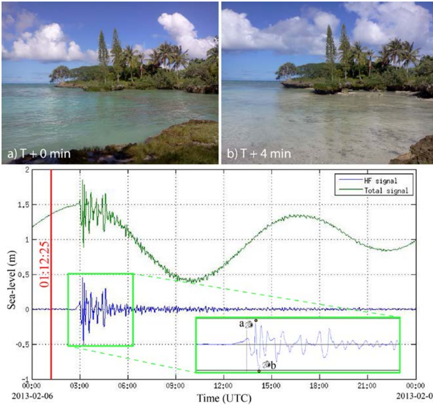
Figure 6 : The February 6, 2013 Solomon tsunami record on Lifou tide gauge (green: raw signal; blue: filtered). The red line locates the earthquake time. The two pictures have been taken at Mou (on the South-eastern coast of Lifou) at the maximum (a) and minimum (b) sea levels and located on the green inset focusing on the main tsunami signal (Photos courtesy of Matthieu Le Duff).
