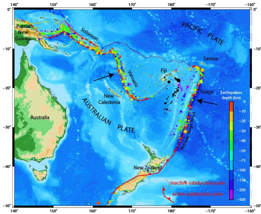
450 Figure 1: Regional tectonic settings around New Caledonia. The colored dots represent M_w \geq 6.0 earthquakes recorded since January 01, 1900 and their sizes are function of magnitude. The black arrows symbolize the relative motion of the Australian and Pacific plates (cm/yr).
