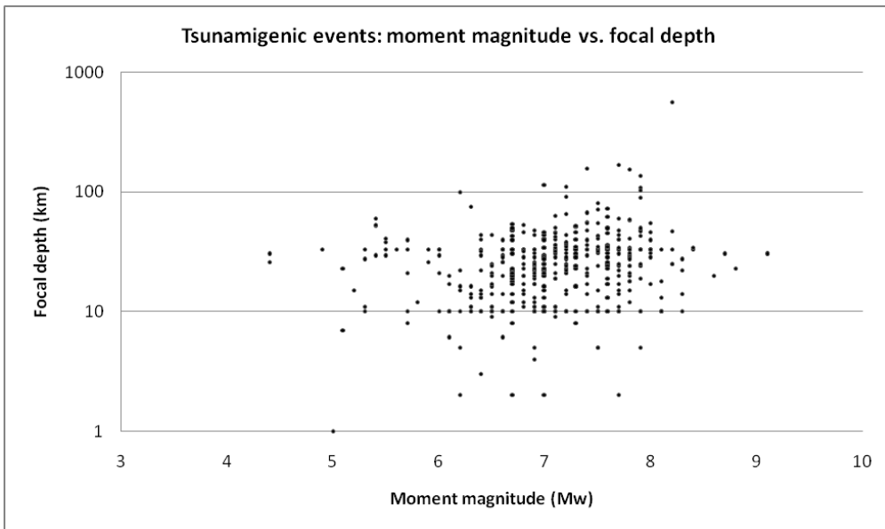
Figure 2 : Relationship between earthquake focal depth and moment magnitude for 440 tsunamigenic events of the NGDC/WDS Global Historical Tsunami Database.
