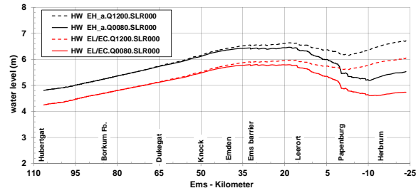
Figure 9. Highest water level levels along a longitudinal profile in the Ems estuary during EH_a (black lines) and EL/EC (red lines) for Q=80 \text{ m}^3 \text{ s}^{-1} (solid lines) and Q=1200 \text{ m}^3 \text{ s}^{-1} (dashed lines) for an open storm surge barrier without SLR.
