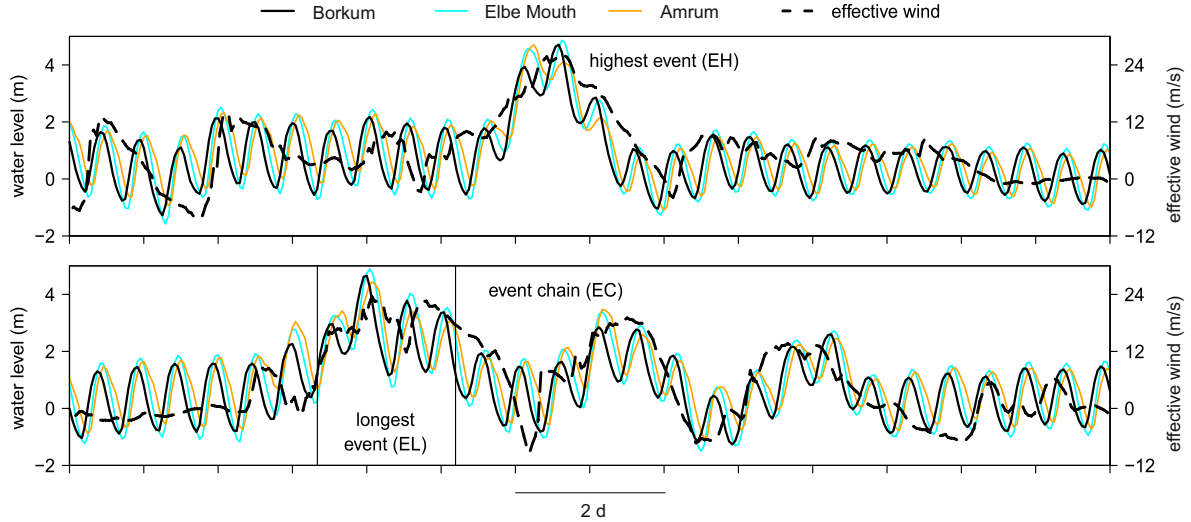
Figure 4. Time series of simulated hourly -water levels for three locations along the German Bight coast together with effective wind velocities for Borkum (dashed black) for the "highest" event (EH, top) and the "event chain" (EC, bottom) over 14 days. The first event in the event chain represents the "longest" event (EL).
