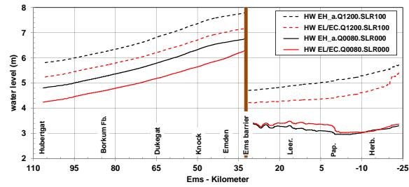
Figure 11. Highest water level levels along a longitudinal profile in the Ems estuary for an operated storm surge barrier without further amplification ( Q=80 \text{ m}^3 \text{ s}^{-1} , \text{SLR}=0 \text{ cm} ; solid lines) and a simulation with enhanced amplified conditions ( Q=1200 \text{ m}^3 \text{ s}^{-1} , \text{SLR}=100 \text{ cm} ; dashed lines) for EH_a (black lines) and EL (red lines).
