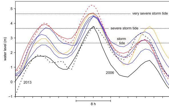
Figure 3. Time series of hourly -water levels over 36 h for Borkum. The two black curves display observations (Data source: "German Federal Waterways and Shipping Administration (WSV)", communicated by the German Federal Institute of Hydrology (BfG)) and the coloured curves represent the five highest simulated storm tides (nearest seaward grid point to Borkum) from the data set. The red and the orange curves denote the two highest events (EH and EL) used for amplification tests, the dashed red curve displays the amplified event EH_a (see chapter 3.1.2).
