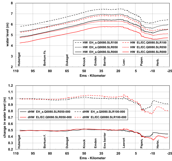
Figure 10. top: Highest water level levels along a longitudinal profile in the Ems estuary during EH_a (black lines) and EL (red lines) for SLR=0 cm (solid lines), SLR=50 cm (dotted lines) and SLR=100 cm (dashed lines) for an open storm surge barrier and Q=80 \text{ m}^3 \text{ s}^{-1} . bottom: Differences in the highest water levels between simulations with and without SLR along the Ems estuary during EH_a (black lines) and EL (red lines) for Q=80 \text{ m}^3 \text{ s}^{-1} (dashed lines for SLR=100 cm, solid lines for SLR=50 cm). The storm surge barrier is open.
