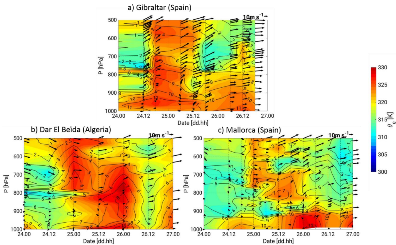
840 Figure 5. Time-height cross-sections at Gibraltar (a), Dar el Beïda (b) and Mallorca (c) between 24-Oct 0000UTC and 27-Oct 0000UTC. The colour shading stands for Equivalent Potential Temperature ( \theta_e ), the contours denote specific humidity and the arrows show the direction and speed of horizontal wind at the stations. The location of the radiosondes can be seen in Fig. 1.
