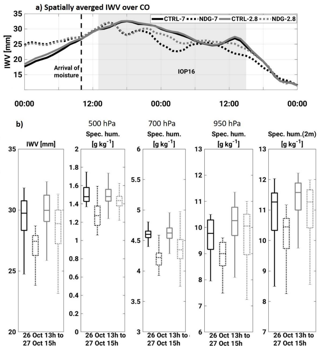
870 Figure 9. Spatially averaged I WV for all simulations during the event. The area for averaging is shown in Fig. 1 (CO) and the model output has been upscaled to a common coarser grid. The period shown is 26-Oct 0000 UTC to 28-Oct 0000 UTC. (b) Box and whiskers plots showing the median, the percentiles 25 and 75 and the extreme values of I WV and specific humidity at 500 hPa, 700 hPa, 950 hPa and at 2m height. All box and whiskers are obtained from the distribution of values for the shown quantities between the 26-Oct 1300 UTC and 27-Oct 1500 UTC over the study region CO.
