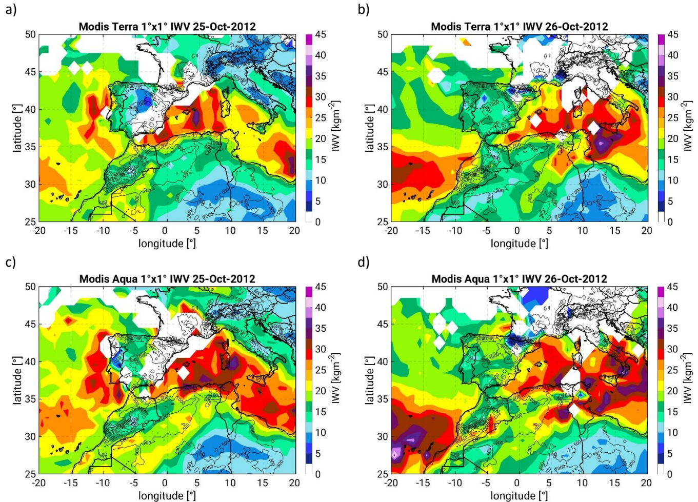
Figure 1. Daily averaged IWV measured MODIS onboard Terra (a, b) and Aqua (c, d). The spatial resolution is 1^\circ \times 1^\circ . The products used are MOD08_D3 and MYD08_D3.
