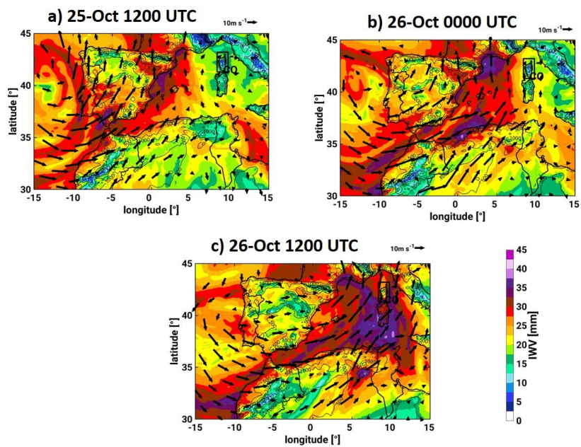
Figure 4. Spatial distribution of IWV and winds at 850 hPa as represented by CTRL-7 on the 25-Oct-2012 at 1200UTC (a), 26-Oct 0000UTC (b) and on the 26-Oct-2012 at 1200UTC (c).
