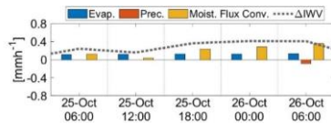
Figure 7. —Temporal evolution of the moisture budget terms, variation of IWV ( \Delta IWV ), Moisture Flux Convergence, Evapotranspiration and Precipitation. Hourly values are given. The spatial averages are performed over the investigation areas NA (a) and MED (b). The values are obtained from CTRL-7.
