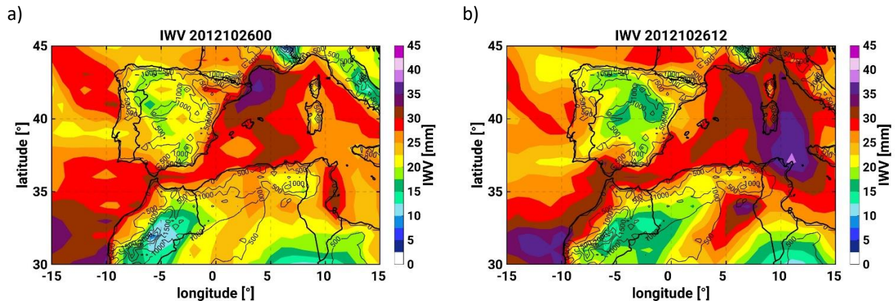
Figure 2. IWV simulated by GDAS on the 26-Oct-2012 at 0000 UTC (a) and at 1200 UTC (b).
