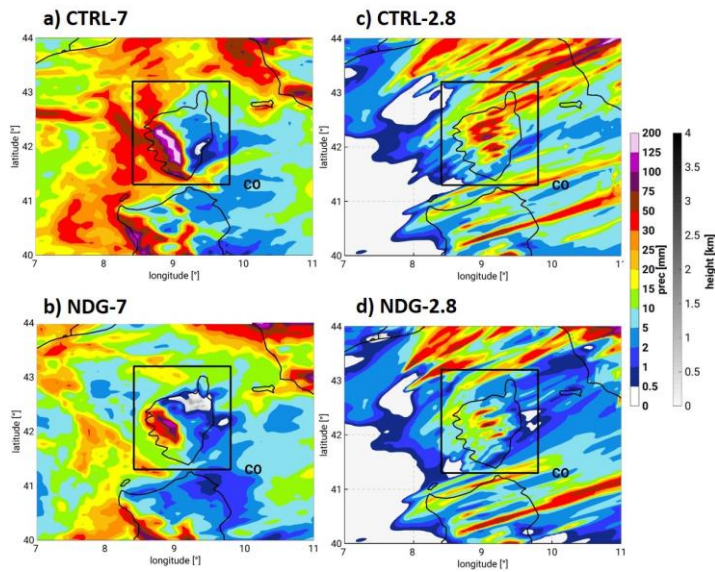
Figure 8. COSMO-CLM accumulated precipitation over Corsica between 26-Oct 1300 UTC and 27-Oct 1500 UTC i.e. during the period of precipitation over the island.
