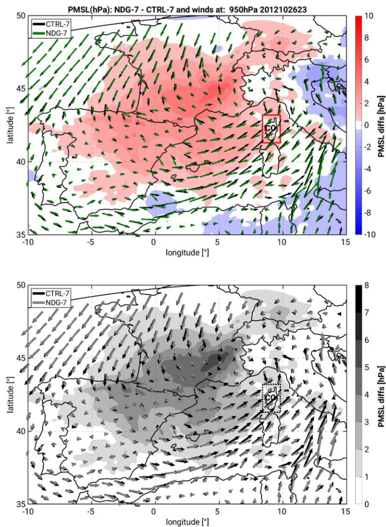
905 Figure 13. Spatial distribution of the differences in Pressure at the Mean Sea Level (PMSL) between NDG-7 and CTRL-7 on the 26-Oct 2300 UTC in a grey scale. Darker grey/Red colours indicate larger PMSL in NDG-7. Horizontal winds at 950 hPa are represented by black (CTRL-7) and green-grey (NDG-7) arrows.
