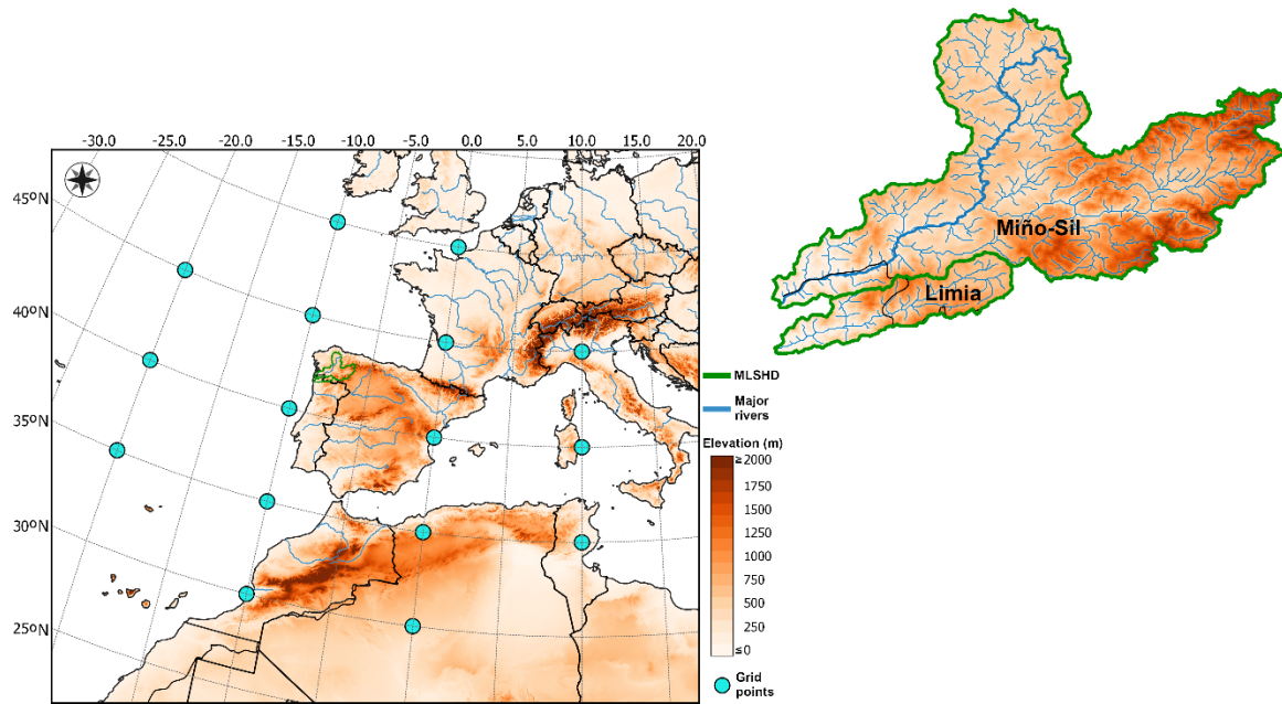
Figure 1. Geographic location and boundaries (green line) of the Miño-Sil and Limia River Basins which conform to the 125 Miño-Limia-Sil Hydrographic Demarcation (MLSHD). The rivers are represented by blue lines and elevation is shaded in red (in meters above sea level) from the HydroSHEDS project (Lehner et al., 2011). Light blue circles denote the location of the 16 points used to retrieve daily MSLP values for the circulation weather types (CWTs) computation.
