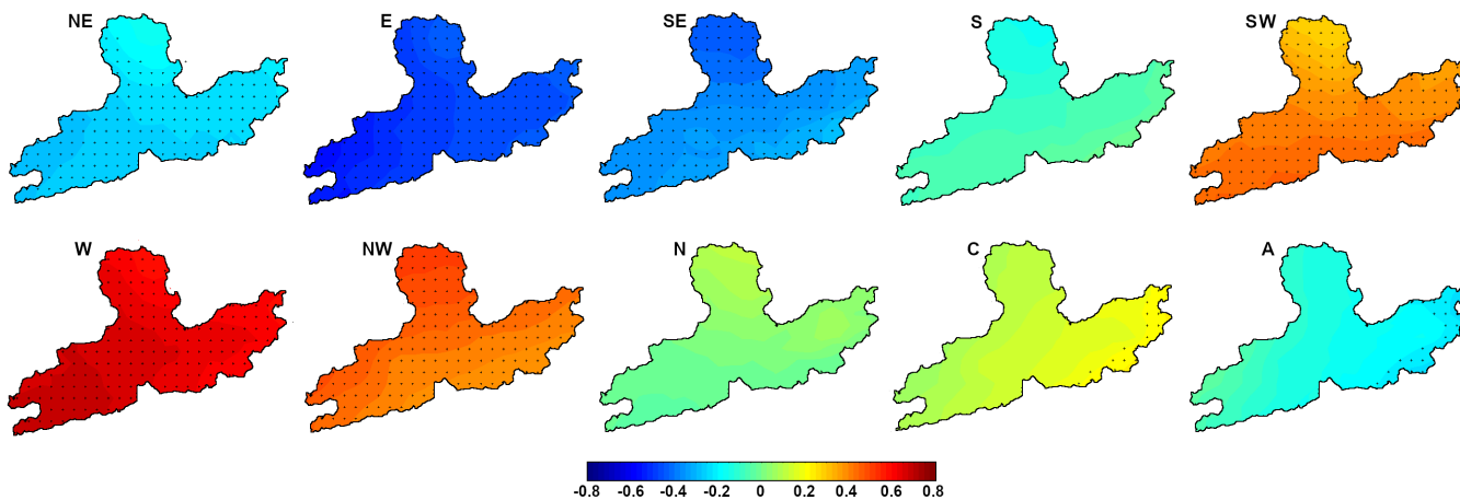
Figure 10. Spatial correlations between detrended grid series of SPEI1 at a resolution of 0.1^\circ in longitude and latitude, and detrended monthly percentages of occurrence of each of the pure CWTs for 1980–2017. The dots in every correlation map denote statistically significant correlations at p < 0.05 .
