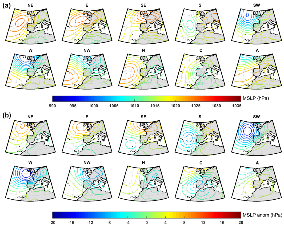
465 Figure 8. (a) Mean sea level pressure (MSLP) fields; and (b) anomaly fields' configuration of the 10 pure circulation weather types (CWTs) for the period 1980–2017. The contour interval is 2 hPa.
