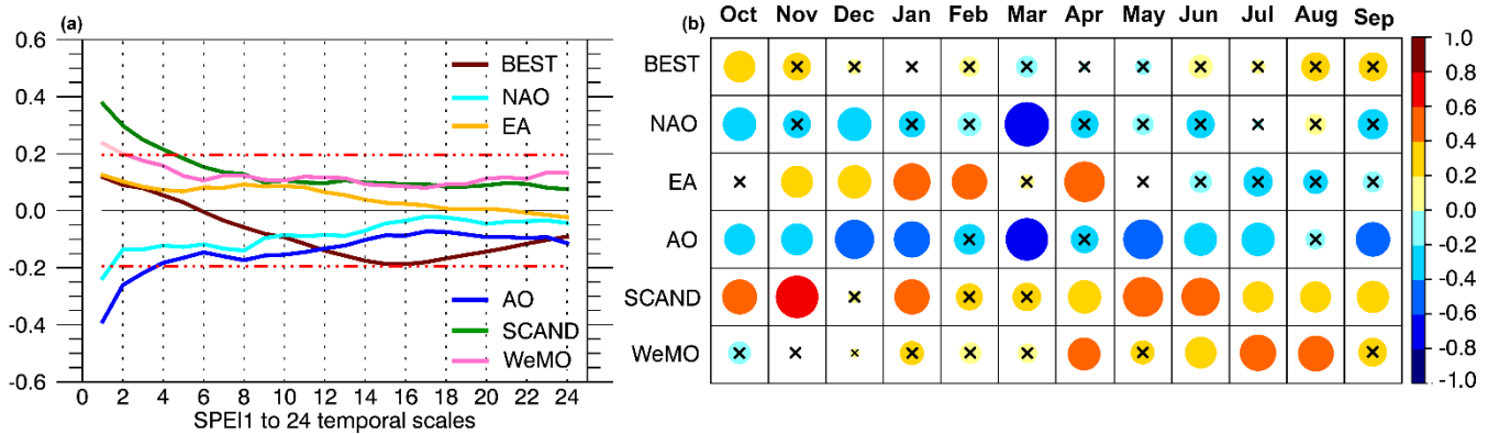
Figure 15. Correlation between the monthly series of the bivariate El Niño Southern Oscillation (BEST), North Atlantic Oscillation (NAO), East Atlantic (EA), Arctic Oscillation (AO) and Scandinavian Pattern (SCAND) and (WeMO) with (a) monthly series of the SPEI1 to SPEI24; and (b) the monthly correlation between the same climatic indices and the SPEI1 for the period 1980–2017. Statistically non -significant correlations at 95% confidence level are those within discontinuous red lines in (a) and marked with an "x" in (b). The size of each circle is proportional to the correlation value.
