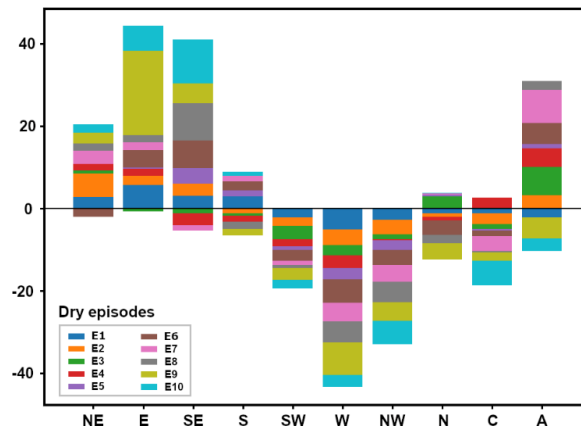
585 Figure 13. Anomalies in the percentage of each CWT associated with the 10 most severe drought episodes listed in Table 3.
