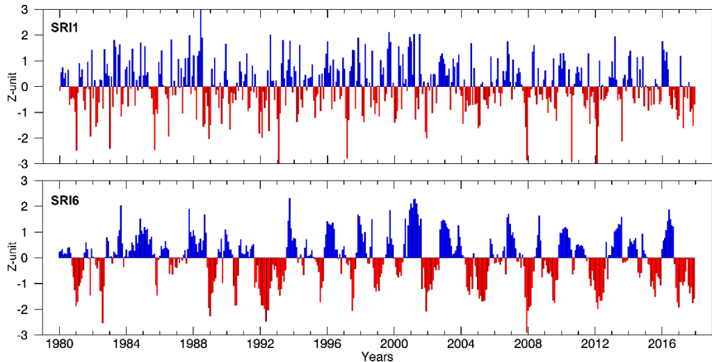
780 Figure 17. Temporal evolution of the Standardised Runoff Index computed for (a) 1-month; and (b) 6-month temporal scales in the MLSHD. Period 1980–2017.
