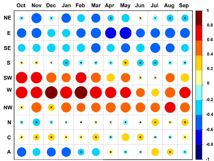
530 Figure 9. Correlations between the detrended series of SPEI1 and the monthly percentage of occurrence of each of the pure weather types CWT for 1980–2017. The size of the circles is proportional to the correlation values. The x's inside the circles represent non -statistically non -significant correlations at p < 0.05 .
