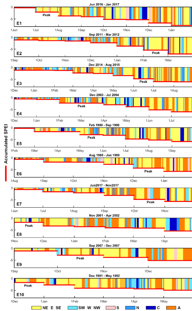
575 Figure 12. Accumulated SPEI1 (red line) and grouped CWTs during the 10 most severe drought episodes listed in Table 3.
