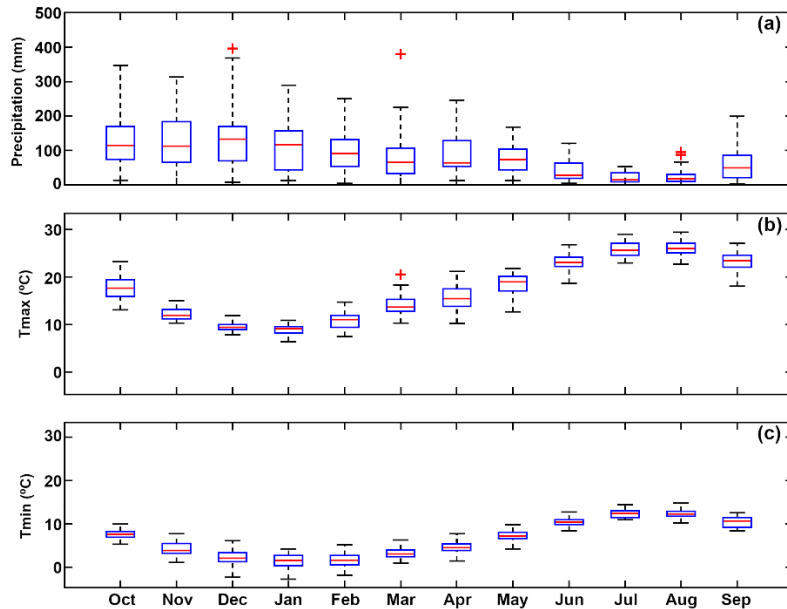
180 Figure 2. The annual cycle for the hydrological year spanning October of year n to September of year n+1 , for the period 1980–2017, of (a) monthly mean precipitation; (b) maximum temperature; and (c) minimum temperature in the MLSHD Miño-Limia-Sil Hydrographic Demarcation , using the E-OBS gridded dataset. Boxes delineate the median (red line), upper, and lower quartiles, with the whiskers representing the lowest and highest monthly value still within 1.5 of the interquartile range. +: outliers, i.e. values beyond the ends of the whiskers.
