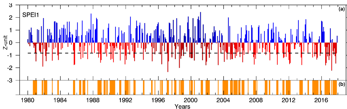
415 Figure 5. Wet (blue bars) and dry (red bars) conditions in the MLSHD according to the (a) SPEI1; and (b) dry episodes (orange bars) during 1980–2017.
