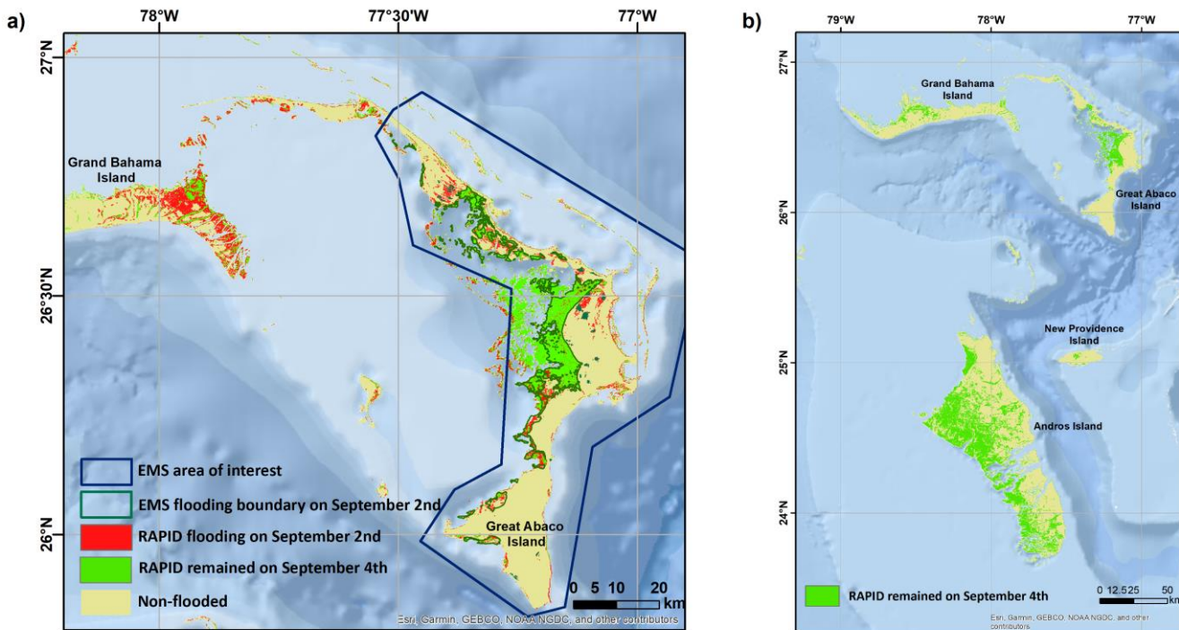
225 Figure 2: a) Flooded and non-flooded areas on September 2 and September 4, 2019 derived from the RAPID algorithm that processed SAR data from the Sentinel-1 overpasses, and flooded boundary on September 2 from Copernicus EMS. b) RAPID flooding map for the entire Northern and Central Bahamas, for the September 4, 2019 Sentinel-1 overpass. For both images, ocean background from World Ocean Base map (ESRI et al. 2014; list of contributors available at: http://downloads.esri.com/esri_content_doc/da/WorldOcean_ContributorsDA64.pdf ).
