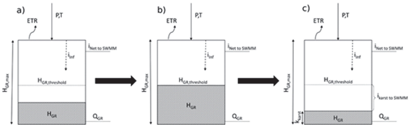
15 Figure S2 Schema of the modified infiltration model including a karstic component. Only the relevant parameters are shown.
