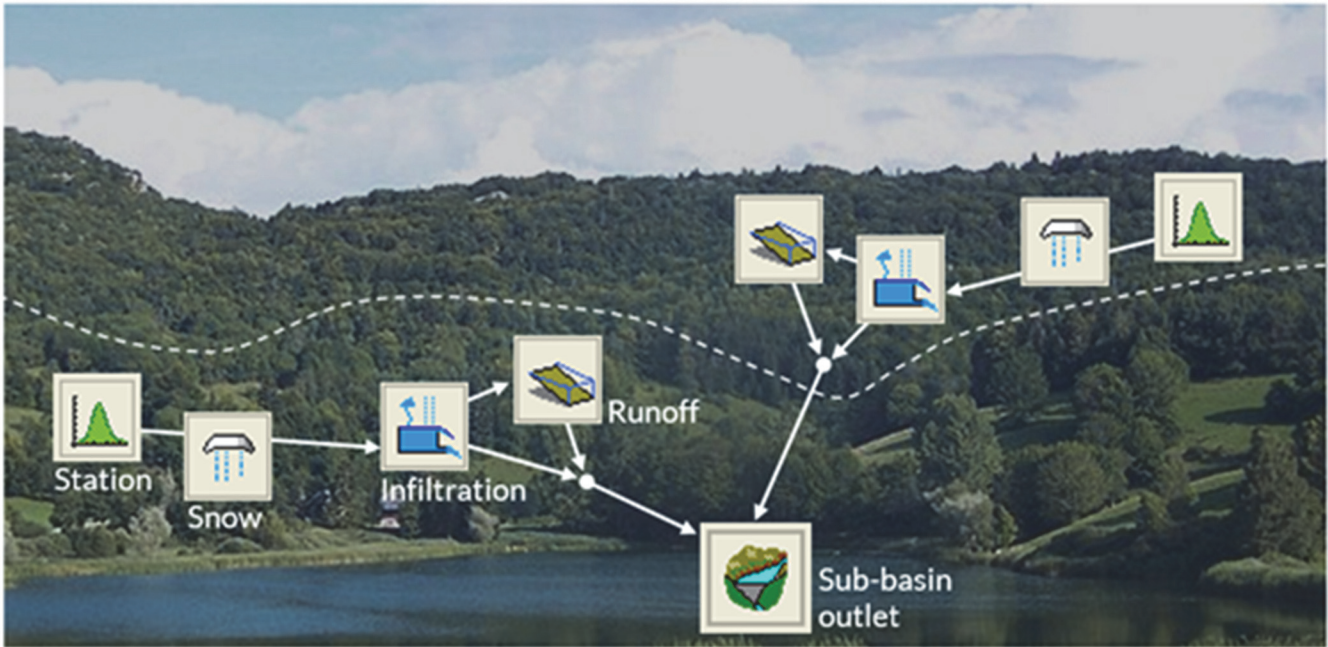
10 Figure S1 Semi-distributed rainfall-runoff modelling with GSM-SOCONT. The sub-basins is divided in two elevation bands in this example.
