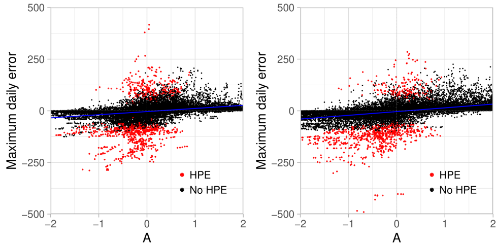
Figure 1: Relationship between the daily rainfall gridpoint maximum algebraic error and the A-component of the SAL score. HPEs days are plotted in red, while other days are in black. Left panel is for LT12 lead time, right panel shows LT34 lead time. Linear regression analysis is added to the plot.
