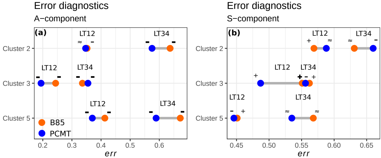
Figure 10. Dumbbell plot of integrated error diagnostics computed using eqEq. 11 . Colours refer to B85 (orange) and PCMT (blue) deep convection parametrization schemes. Results are stratified on the basis of the clusters and lead times. Symbols denote whether positive or negative errors dominate. These signs are defined using the following definition: - (bold) if \frac{err_-}{err_+} \geq 2 ; - if 1.1 \leq \frac{err_-}{err_+} < 2 ; \approx if 0.9 < \frac{err_-}{err_+} < 1.1 ; + if 0.5 < \frac{err_-}{err_+} \leq 0.9 ; + (bold) if \frac{err_-}{err_+} \leq 0.5 .
