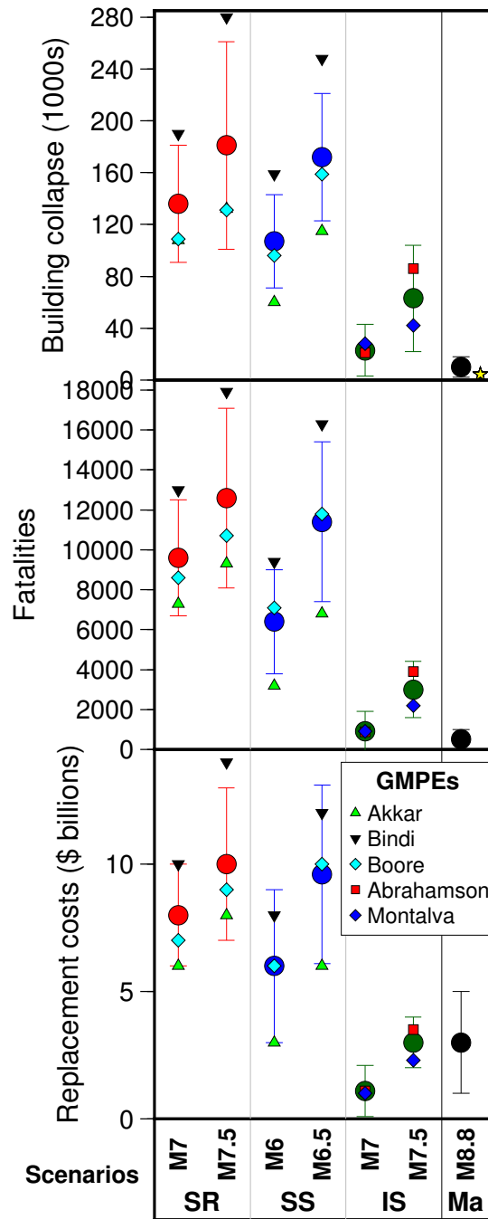
Figure 11. A summary of the total number of building collapse, fatalities and replacement costs for each scenario calculation. The solid circles are the average across the GMPEs considered in each scenario, which are indicated by the smaller polygons. The spread in the estimates from the GMPEs indicate the epistemic uncertainty in our calculations. Error bars represent 1 standard deviation determined from the 1000 Monte Carlo simulations. The yellow star denotes the actual number of building collapses (4,306) in Santiago in the 2010 Maule earthquake (Elnashai et al., 2010).
