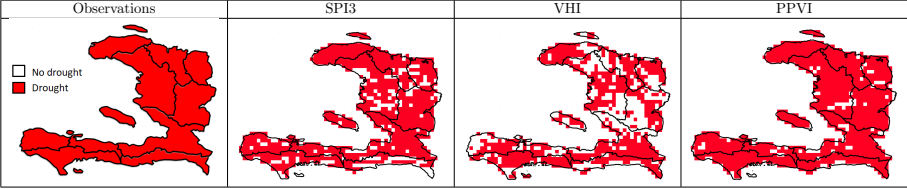
Figure 9. Same as Fig. 7.8 but for week 33 of 2015. Departments highlighted in red are the ones in drought according to observations, black red cells are the ones in drought condition according to the various indices.
