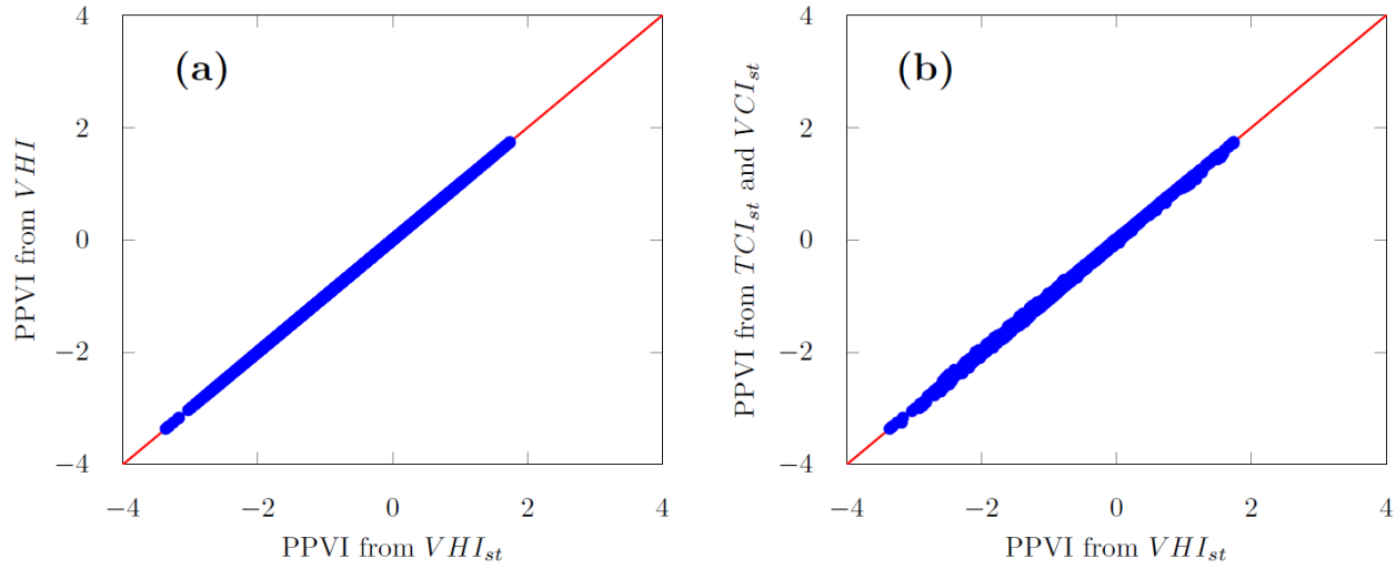
Figure 1: (a): relationship between PPVI computed from VHI_{st} and PPVI computed from VHI; (b): relationship between PPVI computed from VHI_{st} and PPVI computed from VHI_{st} retrieved from linear combination of VCI_{st} and TCI_{st} .
