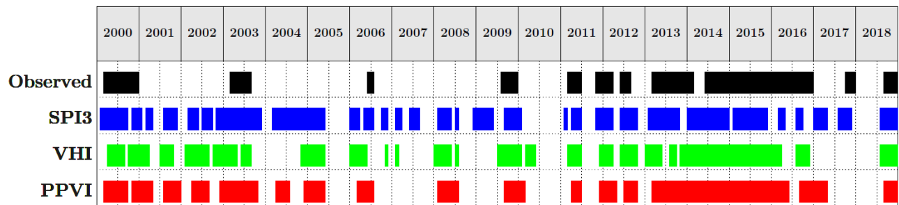
Figure 2: comparison between observed drought events and drought events identified by PPVI, SPI3 and VHI when calibrated with the best performing parameters shown in Table 10. The comparison is shown for the period from 2000 to 2018.
