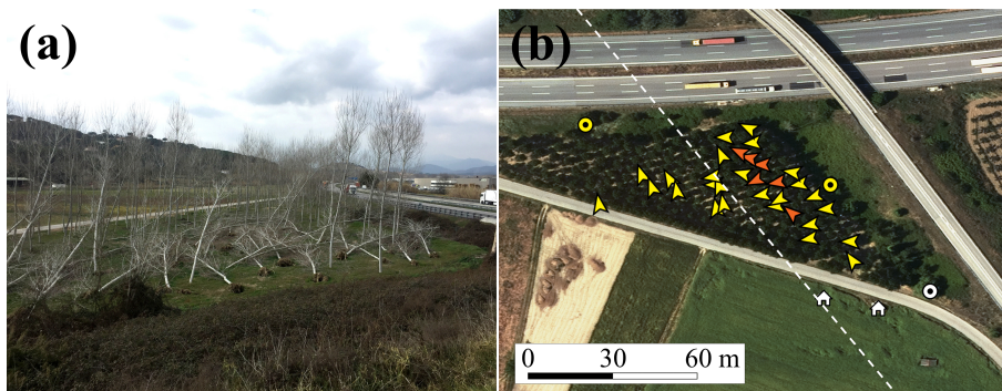
Figure A2. (a) A poplar plantation from Fogars de la Selva (Catalonia) affected by the 15 October 2018 EF1 Malgrat de Mar – Massanes tornado, and (b) fallen trees directions of the same poplar plantation. Map symbols indicate locations of damage in man-made structures (house icon) and fallen tree or damaged vegetation element (arrow or circle icon if no direction is available). Icon colours indicate damage intensity: EF0 (yellow), EF1 (orange) and unrated (white). The white discontinuous line separates the right-half and the left-half sides of the damage swath where predominant fall tree direction are west and north, respectively. The background orthophoto is from the Institut Cartogràfic i Geològic de Catalunya (ICGC), http://www.icc.cat (last access: September 2019), under a CC BY 4.0 license.
