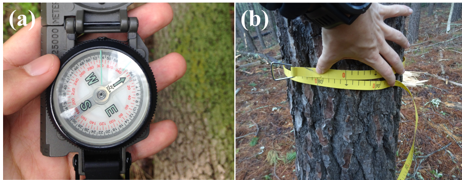
Figure 5. (a) Measure of the fall direction of a tree and (b) measure of trunk diameter during the damage survey of an EF1 tornado on 13 October 2016 in Llinars del Vallès (Catalonia) and an EF2 tornado on 7 January 2018 in Darnius (Catalonia), respectively (Author: Oriol Rodríguez).
