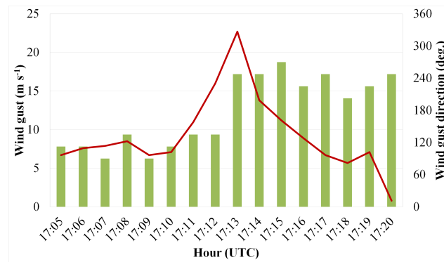
Figure 4. Wind gust (red line) and wind gust direction (green bars) registered by an AWS in Mataró (Catalonia) with 1 minute temporal resolution data. The AWS was located 240 m west of the estimated centre of the EF0 tornado track, on 23 November 2016. Data source: Meteomar, Consell Comarcal del Maresme.
