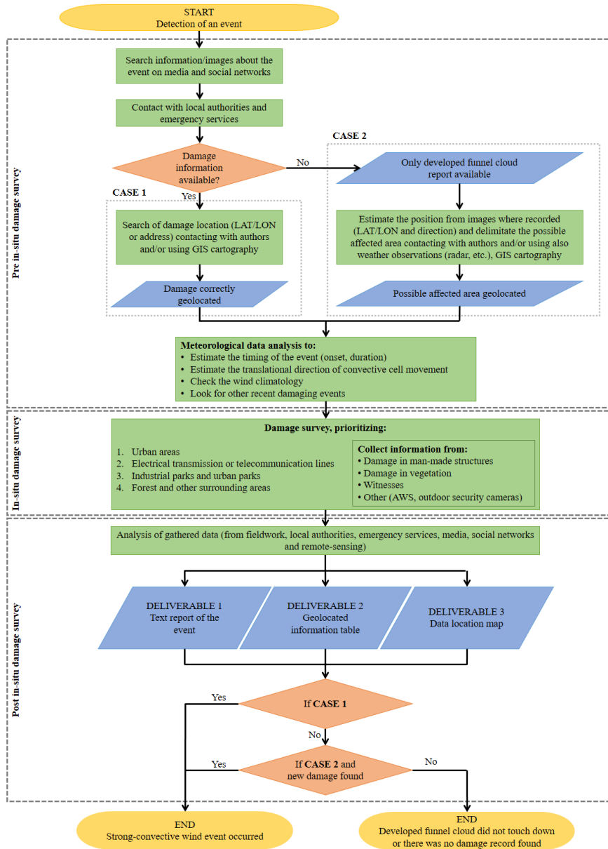
Figure 2. Flow diagram of the structure and application of the proposed methodology to carry out strong-convective winds fieldwork damage assessment. Start and end are shaded in yellow, processes in green, decisions in orange and inputs/outputs in blue.
