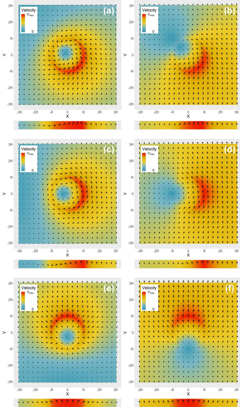
Figure. Two dimensional near surface horizontal wind fields and damage swaths for the cases (a) G=4 and \alpha=45^\circ , (b) G=4 and \alpha=90^\circ , (c) G=4 and \alpha=180^\circ , (d) G=1 and \alpha=45^\circ , (e) G=1 and \alpha=90^\circ , and (f) G=1 and \alpha=180^\circ . Adapted from Figures 3 and 4 of Bech et al. (2009) .
