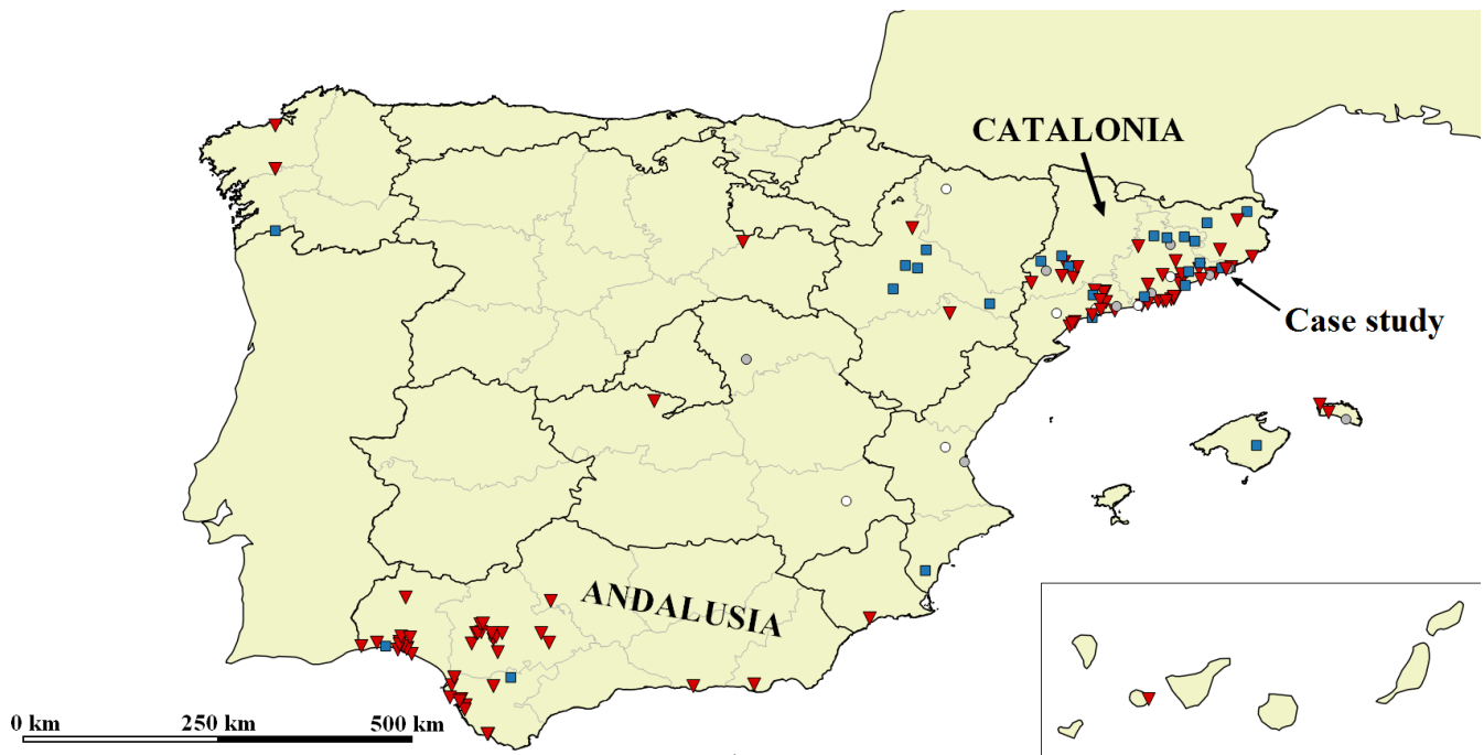
615 Figure 1. Location of 136 analysed events using the proposed methodology between 2004 and 2018, mostly concentrated in Andalusia and Catalonia. Symbols indicate locations of tornadoes (red triangles), downbursts (blue squares), undetermined phenomena (grey circles) and other phenomena such as gust fronts, funnel clouds which did not touch down, or dust devils (white circles). The case study location for which final deliverables are attached as Supplementary material is indicated on the map.
