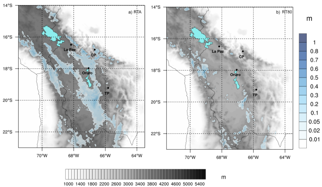
Figure S1. As in Figure 6b but for experiments a) RTA and b) RT80. Gray shading represents the modified orography used during each experiment.
