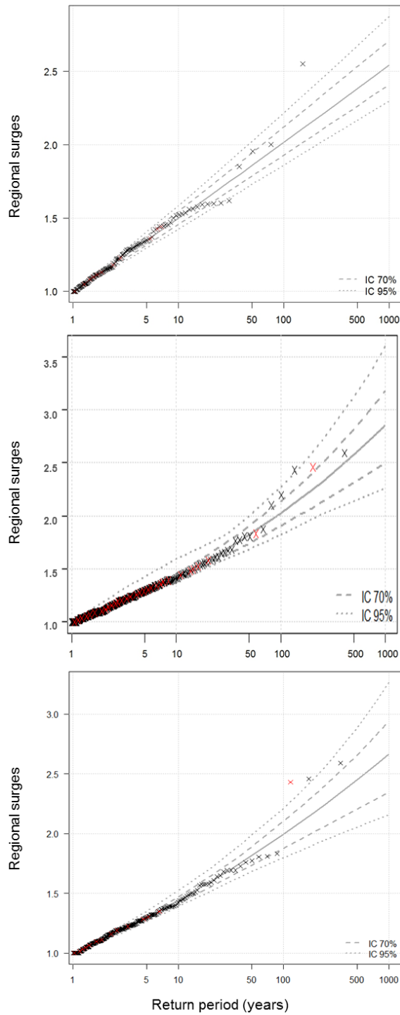
485 Fig. 6. The GPD/sinusoid fitted to regional SSSs (plotting positions, RLs and confidence intervals) for the target sites: Exp_{sin} distribution for Calais (top); GPD_{cos sin} for Brest (middle) and La Rochelle (bottom). The y-axis represent the normalized regional surges (without unit), the x-axis represent the return period (in years). The red crosses indicate the SSSs at the target site, so the black crosses indicate the regional ones. The confidence intervals at 70% (dashed line) and 95% (dotted line), which are computed by the bootstrap method, are also presented (dotted lines).
