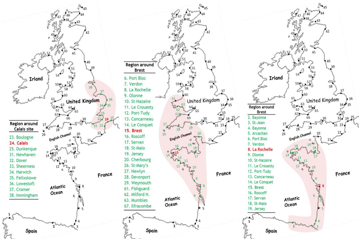
480 Fig. 5. Physically homogenous regions (the list of sites belonging to a region are surrounded by red zones) for Calais, Brest and La Rochelle. Neighbouring sites are represented with green dots (target sites are represented with red dots). Target sites are not close to a border.
