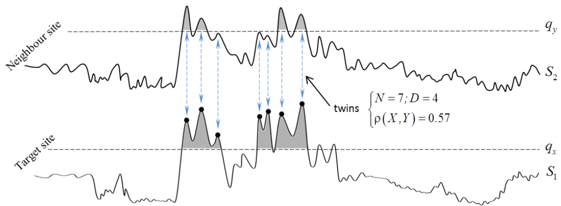
450 Fig. 1. An illustrative example on how the extremal dependency coefficient is empirically computed. Among the 7 extreme twins ( N = 7 ), only 4 overlapped with the target site extreme storm surges ( D = 4 ). The extremal coefficient is then equal to 0.57.
