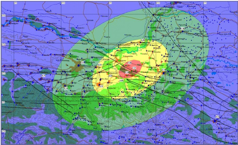
Figure 5: Calibrated model application for simulation the 2008 Kurchaloy earthquake consequences; map based on layers from DCW.
