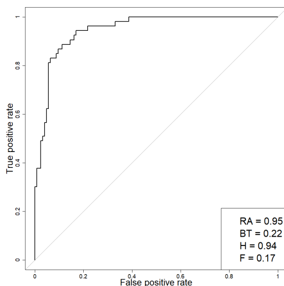
Figure B1. Relative operating characteristic (ROC) diagram for above 70th percentile of damage predictions using Eq. 4 for Catalonia ( P_0=40 mm/24 h). Each value of the ROC curve indicates a set of probability forecasts by stepping a decision threshold with 1 % probability through the modelling results. The numbers inside the plot are the ROC area (RA) and the best threshold (BT), here defined as the threshold that maximises the difference between the hit rate (H) and the false alarm rate (F)
