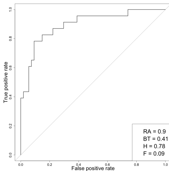
Figure B2. Relative operating characteristic (ROC) diagram for above 70th percentile of damage predictions using Eq. 5 for the Valencian Community ( P_0=40 mm/24 h). Each value of the ROC curve indicates a set of probability forecasts by stepping a decision threshold with 1 % probability through the modelling results. The numbers inside the plot are the ROC area (RA) and the best threshold (BT), here defined as the threshold that maximises the difference between the hit rate (H) and the false alarm rate (F)
