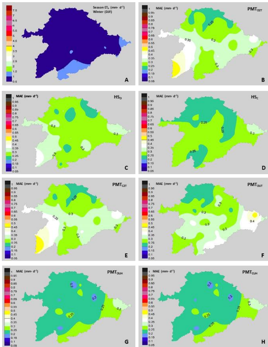
Figure 4. Performance of the models with a winter focus (December, January and February). A, Average values of ET_0 ( mm \cdot d^{-1} ) in winter. Mean values of MAE ( mm \cdot d^{-1} ): B, PMT_{02T} model; C, H_0 model; D, H_e model; E, PMT_{e2T} model; F, PMT_{OUT} model; G, PMT_{OUH} model and H, PMT_{CUH} model
