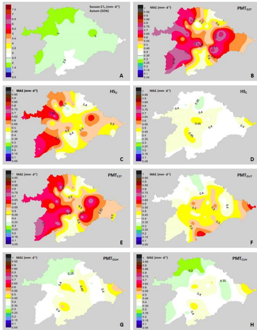
Figure.7. Performance of the models with an autumn focus (September, October and November). A, Average values of ET_0 ( mm \cdot d^{-1} ) in autumn. Mean values of MAE ( mm \cdot d^{-1} ): B, PMT_{O2T} model; C, HS_0 model; D, H_c model; E, PMT_{C2T} model; F, PMT_{OUT} model; G, PMT_{OUH} model and H, PMT_{CUH} model.
