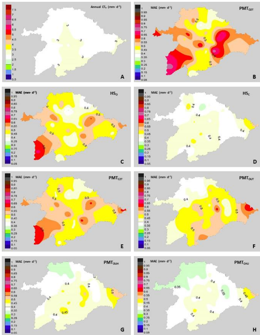
Figure 3. Performance of the models with an annual focus. A, Average annual values of ET_0 (mm·d -1 ). Mean values of MAE (mm·d -1 ): B, PMT O2T model; C, H O model; D, H C model; E, PMT C2T model; F, 375 PMT OUT model; G, PMT OUH model and H, PMT CUH model
