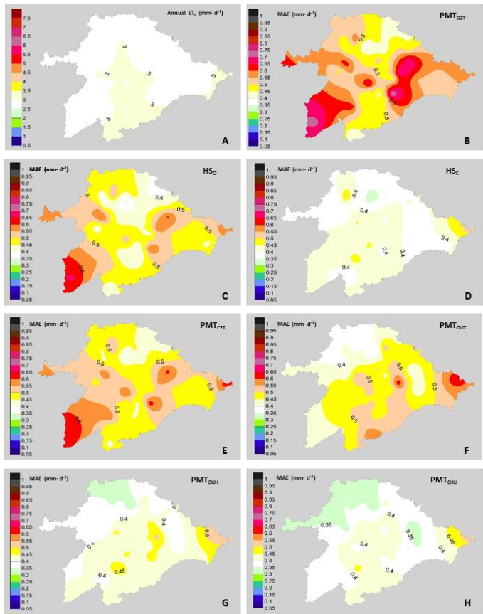
Figure 3. Performance of the models with an annual focus. A, Average annual values of ET 0 (mm·d -1 ). Mean values of MAE (mm·d -1 ): B, PMT O2T model; C, H 0 model; D, H C model; E, PMT C2T model; F, PMT OUT model; G, PMT OUH model and H, PMT CUH model
