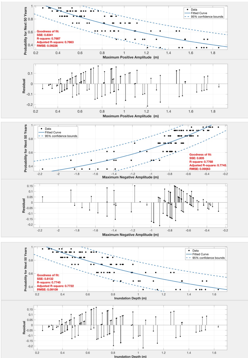
Figure 5: Probabilities of Exceedance Corresponding to Maximum Water Surface Elevation, Minimum Water Surface
