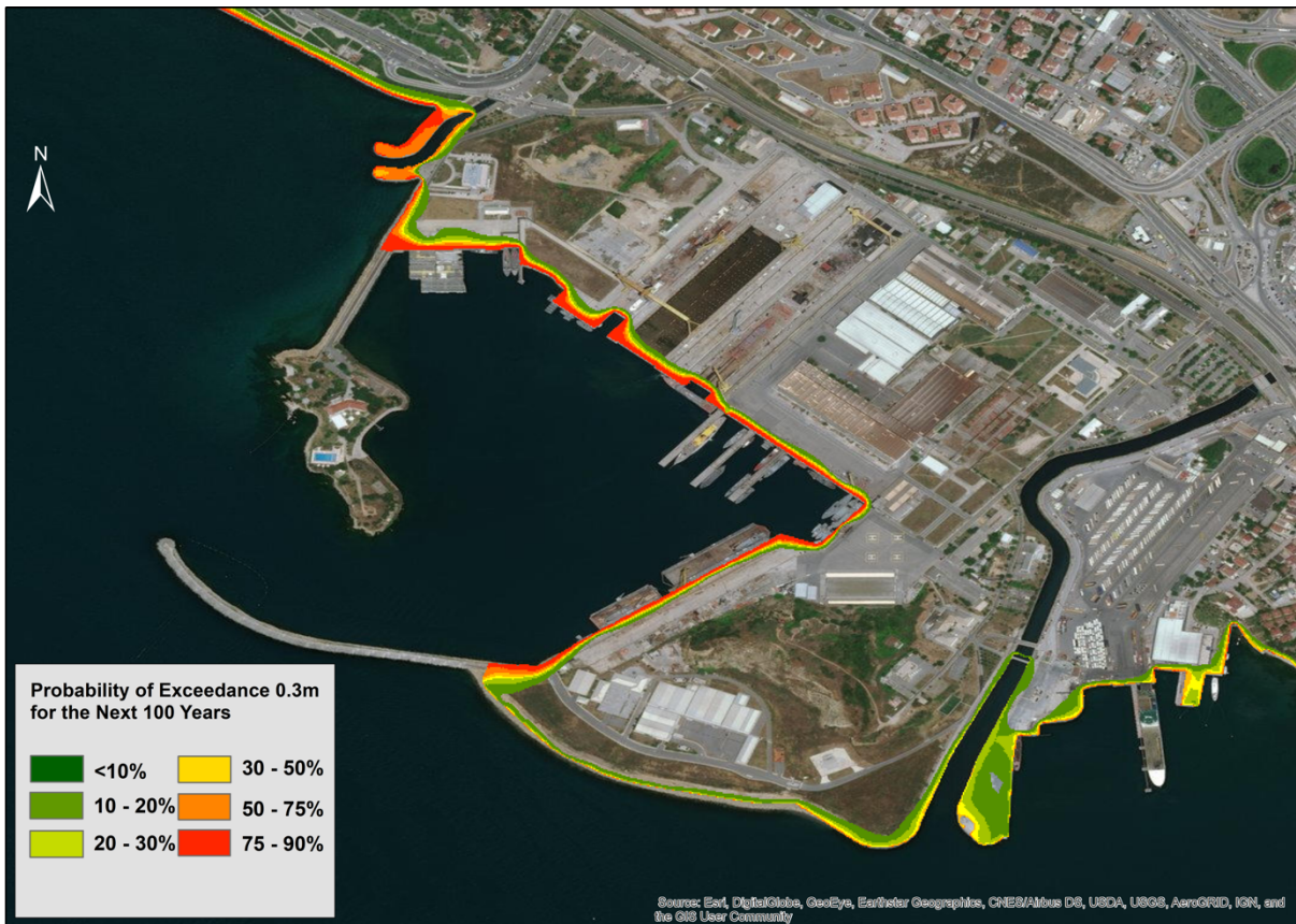
400 Figure 8: Probabilistic Tsunami Inundation Maps of Northern Part of Tuzla Study Domain representing the Probability of Exceedance of 0.3 m Inundation Depth for the Next 50 and 100 Years. Change of colors from green to red represents the increasing probability of exceedance (created using ArcMap Version 10.5).
