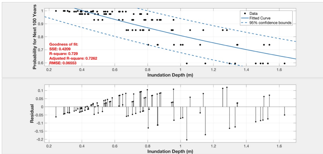
360 Figure 6: Probabilities of Exceedance Corresponding to Maximum Water Surface Elevation, Minimum Water Surface Elevation and Inundation Depth for the next 100 years. Black dots represent the probability of exceedance of tsunami hydrodynamic parameter for each event in the catalog. Blue line is the best fit curve to the data and dashed blue line is the 95% confidence boundary of the fitted curve. Residual of the fit is represented for each probability curve.
