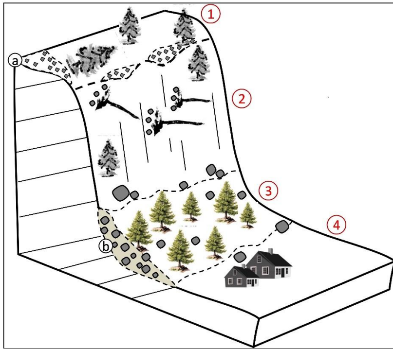
Figure 4: Sketch of the wildfire affected area. During the wildfire, the trees in the less inclined upper rockwall (1) and in the vertical rockwall (2) show indicators for medium fire severity; the protection forest (3) did not get affected by the wildfire. During the fire, rockfalls were detached from the rockface and by falling trees, which reached the houses in the valley floor (4); (a) scree; (b) talus
