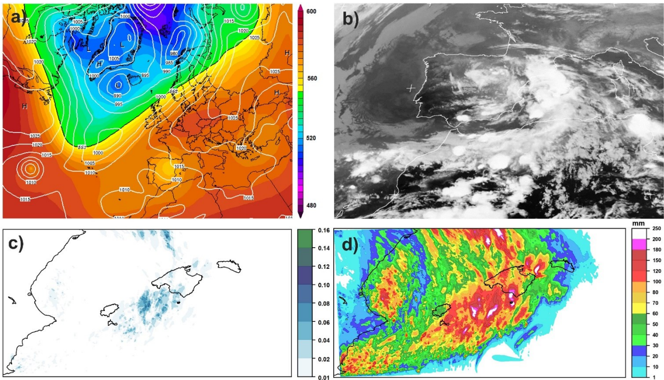
Figure 2. (a) Synoptic situation on October 9, 2018 at 12 UTC (1400h local time) from CFS reanalysis. Colors show geopotential height at 500 hPa (in gpdam according to scale). White contours are isobars (hPa) at sea level (source: https://www.wetterzentrale.de ; CC BY-NC). (b) IR MSG image corresponding to October 9, 2018 at 1700 UTC. (c) Probability of 12h-accumulated precipitation exceeding 100 mm valid at 00 UTC October 10, 2018 from the larger WRF domain initialized at 00 UTC October 9. (d) Maximum 12h-accumulated precipitation across ensemble members valid at 00 UTC October 10, 2018 from the larger WRF domain initialized at 00 UTC October 9.
