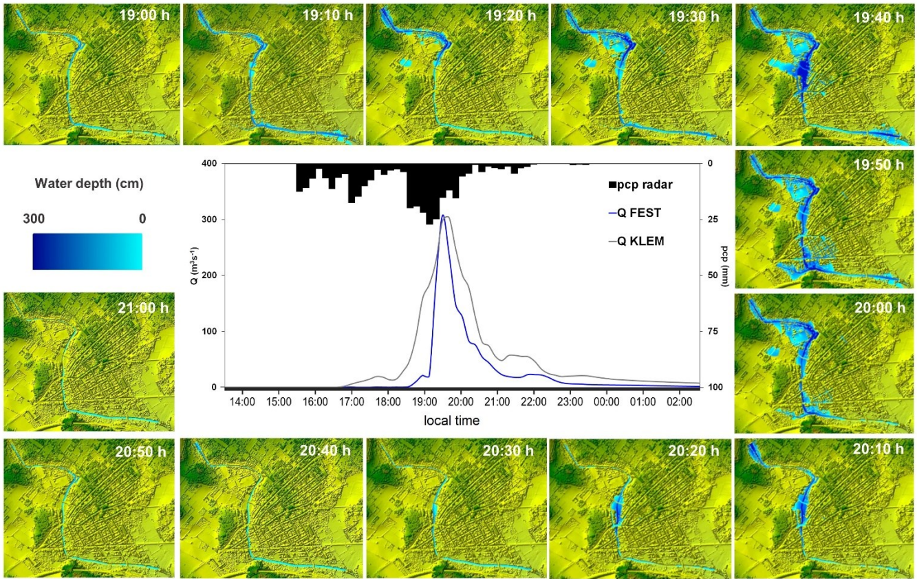
Figure 54. Modelled flash flood hydrograph at the entrance of Sant Llorenç and simulation of the flood peak as it crosses, devastating the town centre between 1900 h. and 2100 h.
