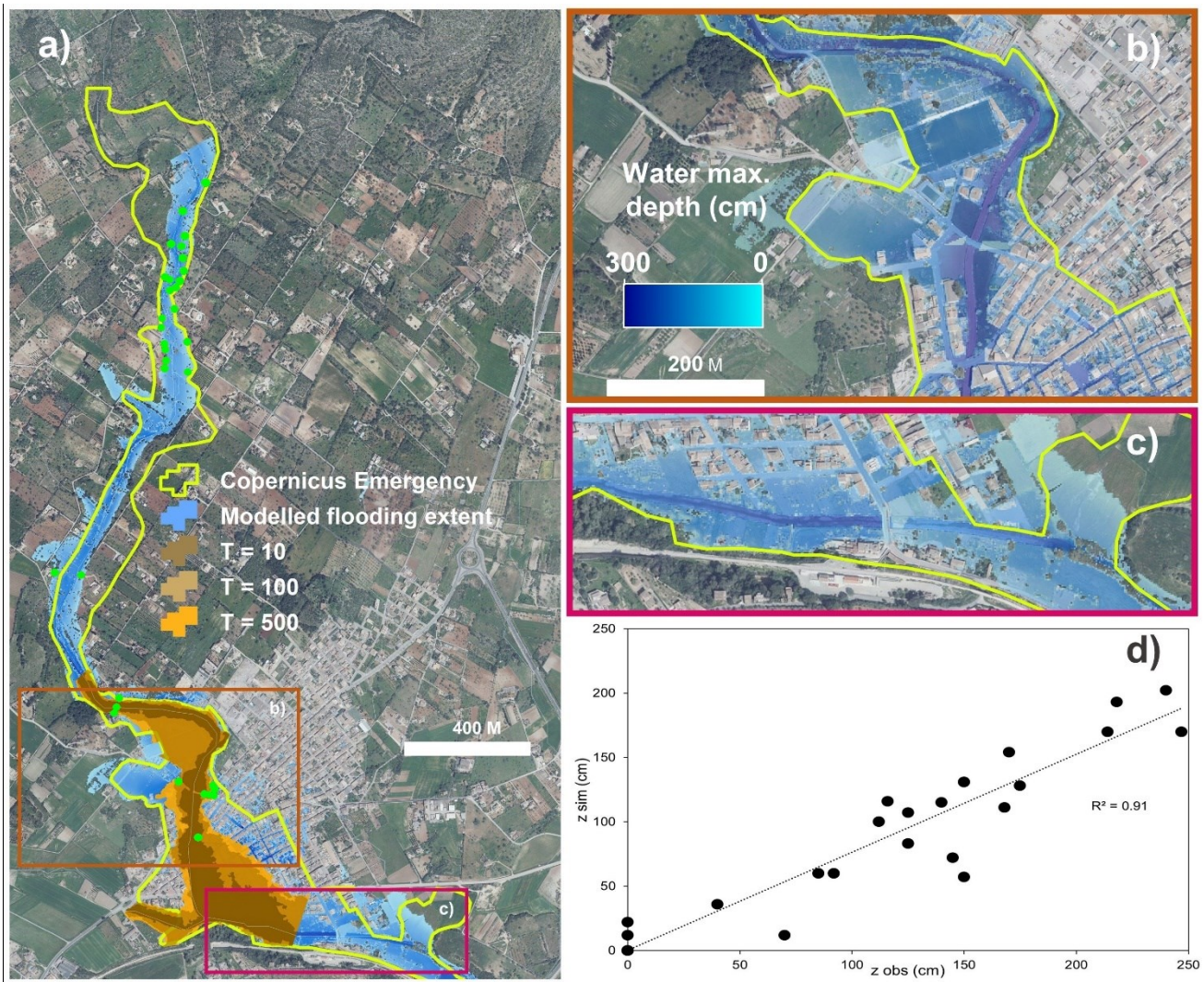
Figure 65. (a) Simulated flooding extent on the village (blue) compared with the observed event by Copernicus Emergency Management System (yellow contour) and selected return periods ( T=10 , T=100 , T=500 ); green dots depict the flooding marks taken as reference to validate the simulation. Detailed views of modelled maximum water depths at Sant Llorenç town (b and c). Scatter plot showing the relationship between simulated water depths and in-situ measured flooding marks (d).
