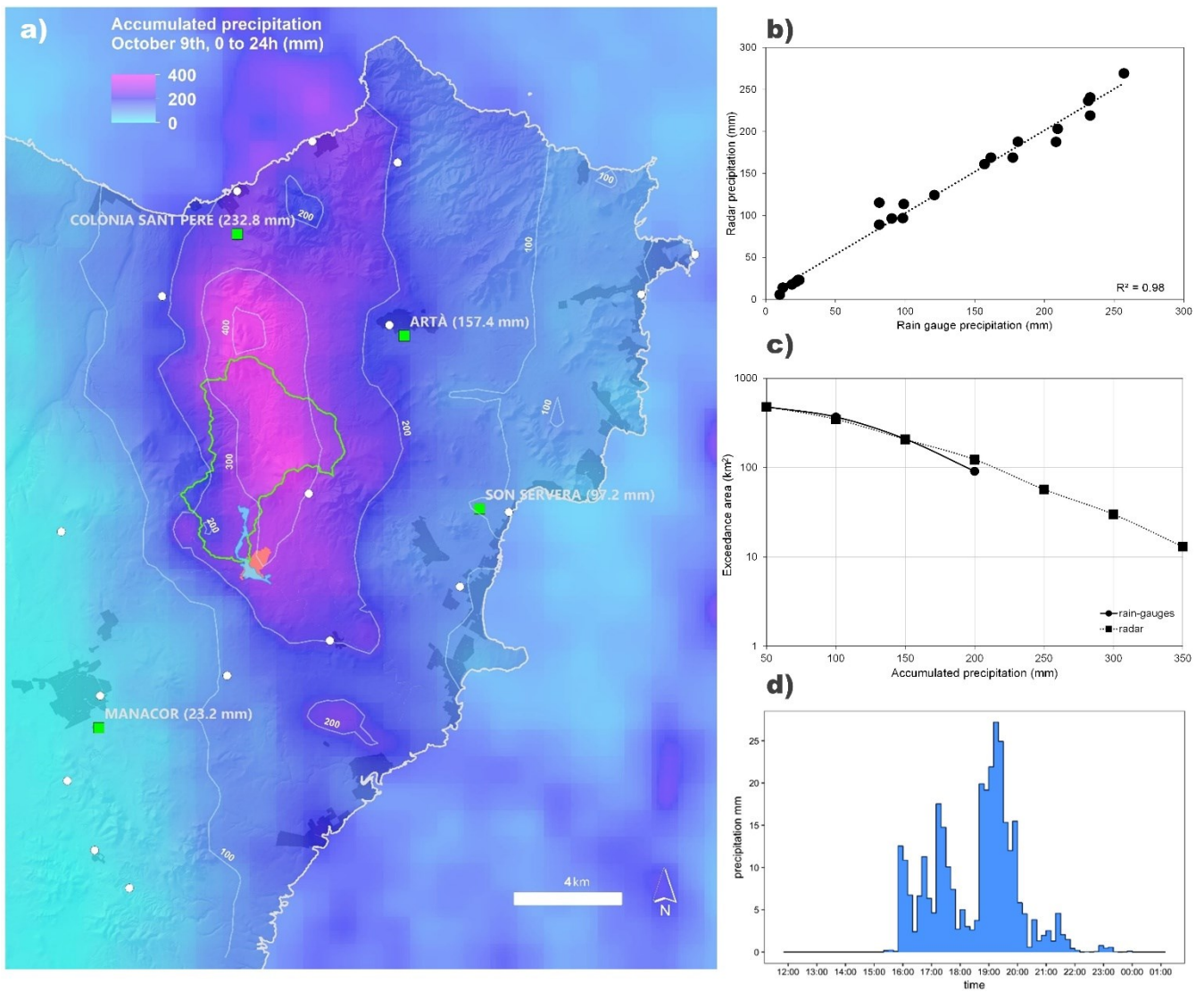
Figure 3. (a) Spatial distribution of the 24-h accumulated radar-estimated precipitation for the October 9, 2018 flash flood. Automatic rain_gauges used for bias correction are shown as squares. Circles depict the daily pluviometric stations. (b) scatterplot of the 24-h accumulated precipitation derived from radar estimates and pluviometric stations. (c) Comparison of the curves of exceedance areas for different rainfall thresholds derived from the 24-h accumulated pluviometric and radar-based rainfall amounts. All pluviometers shown in Fig. 3a have been used for the computation (21 stations). (d) Radar-driven precipitation for the October 9, 2018 episode at Sant Llorenç Ses Planes catchment.
