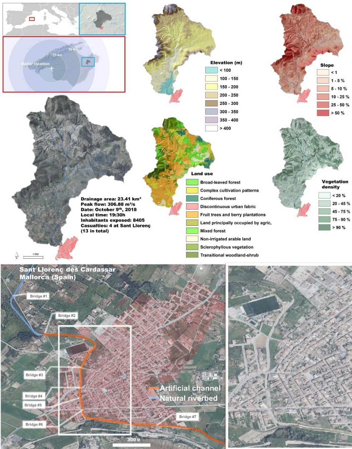
Figure 1. Study area location and overview. Upper panels: characteristics of the contributing watershed at Sant Llorenç (elevation, slope, land cover and LIDAR-derived vegetation density). Lower panels: detailed views of the urban interphase of the torrent de ses Planes at Sant Llorenç des Cardassar.
