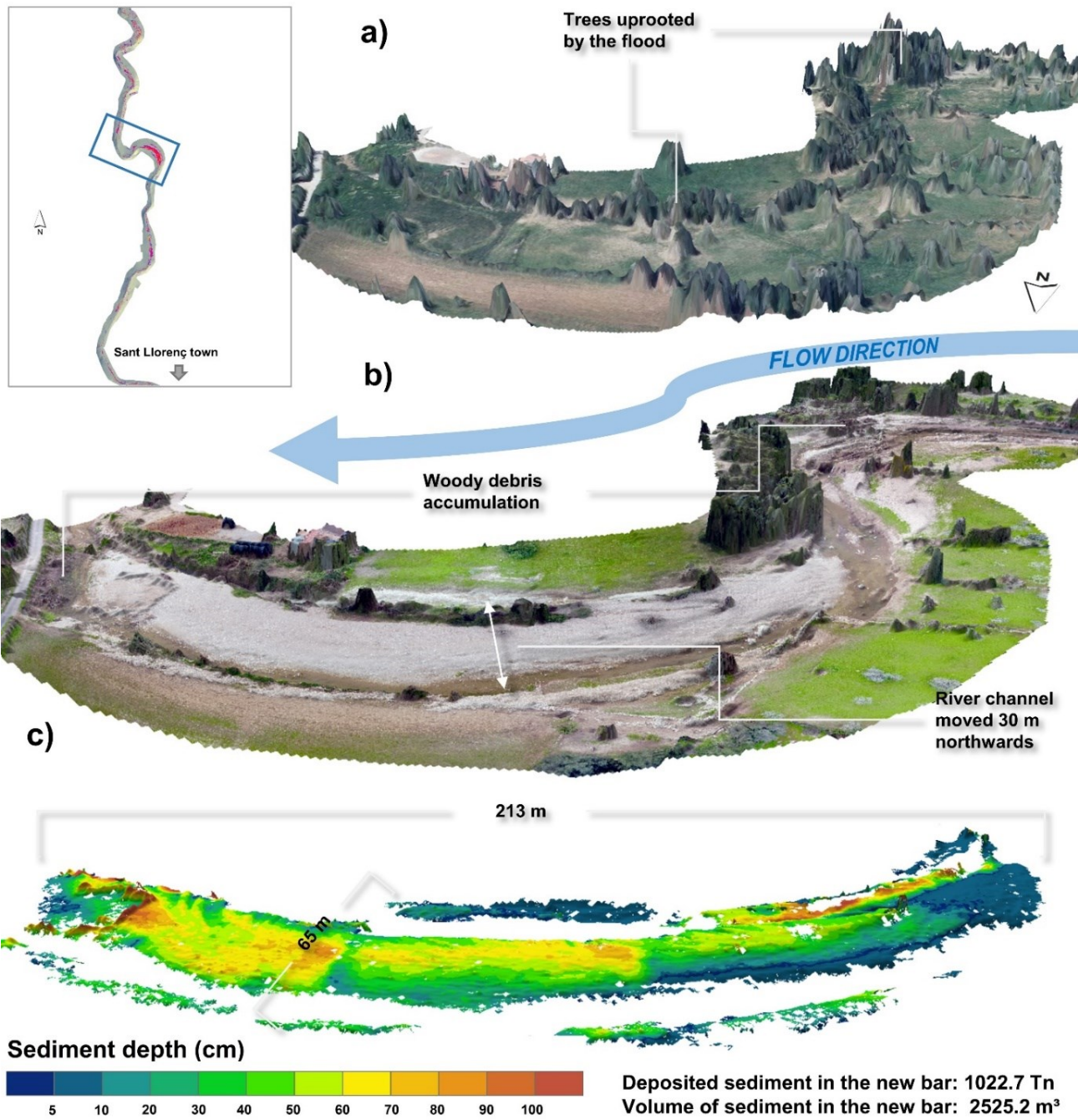
Figure 98. View of the Ses Planes stream at meander 2 km upstream of Sant Llorenç town: December 2014 orthophotograph (25 cm) superimposed onto a LIDAR-derived DEM (1m) before the event (a), and November 2018 orthophotograph (3 cm) dropped onto an SfM-derived DEM (6 cm) after the flash flood (b). Geomorphological changes and details of the sediment bar created during the flash flood at the meander (c).
