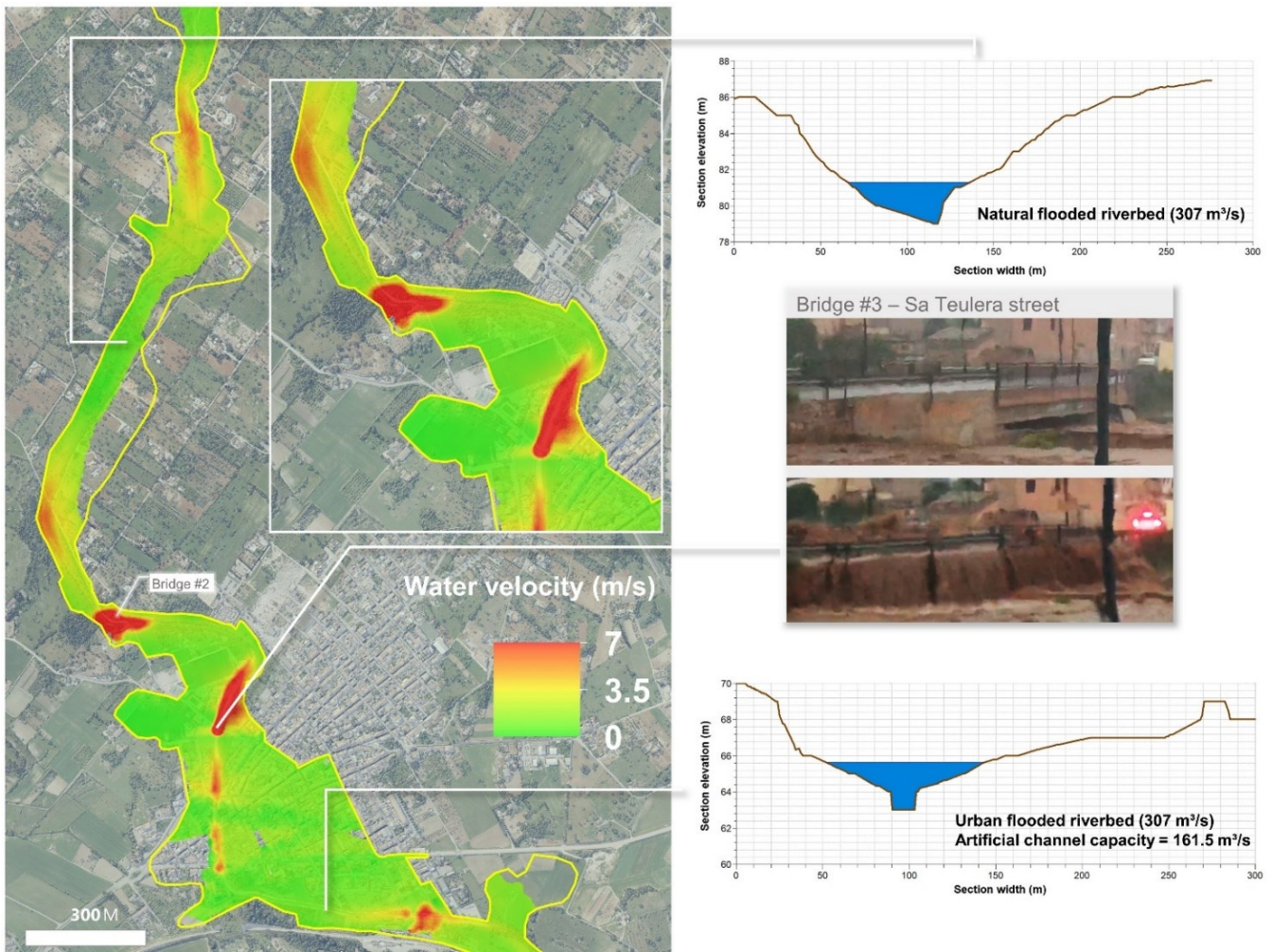
Figure 76. Left panel: simulated maximum water velocity across Sant Llorenç town during the event. Yellow contour line depicts the observed event by Copernicus Emergency Management System. Right panel: maximum discharge flowing through two sections, calculated from flooding marks and LIDAR point clouds, including velocities on the artificial concrete channel.
