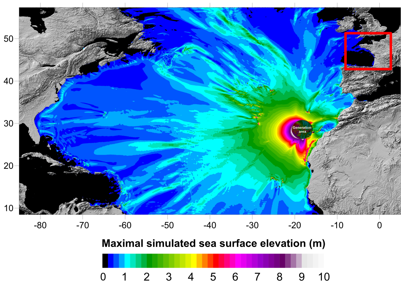
Figure 20. Maximum surface elevations (m) computed by FUNWAVE-TVD for the 80 km 3 scenario, from the generation area to the French coasts and other remote territories, with a 2.7-km resolution. The red rectangle represents a daughter grid covering the western French coasts (see Figures 5 and 21).
