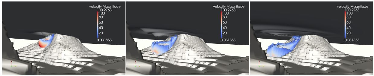
Figure 10. THETIS 3D computations for 80 \text{ km}^3 slide volume. Snapshots of 0.1 slide volume fraction contour colored by velocity magnitude, at : t=100 s (left), 200 s (middle) and 300 s (right). Inviscid slide (Abadie et al., 2012).
