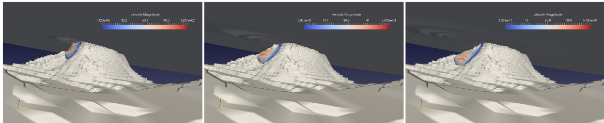
Figure 11. THETIS 3D computations for 80 \text{ km}^3 slide volume. Snapshots of 0.1 slide volume fraction contour colored by velocity magnitude, at : t=102 \text{ s} (left), 230 \text{ s} (middle) and 342 \text{ s} (right). Slide viscosity 2 \times 10^7 \text{ Pa}\cdot\text{s} .
