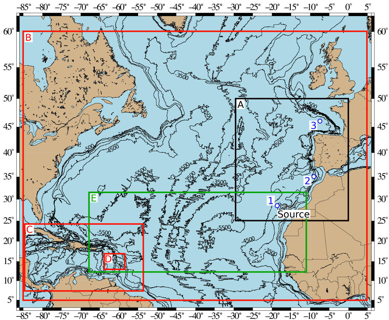
Figure 4. Computational domains for Calypso (2-km (A) resolution in black), FUNWAVE-TVD (2.7 km (B), 930 m (C) and 310 m (D) in red) and SCHISM (in green (E); variable resolution). Bathymetric contours range from -500 m to -7500 m, every 1000 m. Gauges 1, 2 and 3 are marked by white and blue points.
