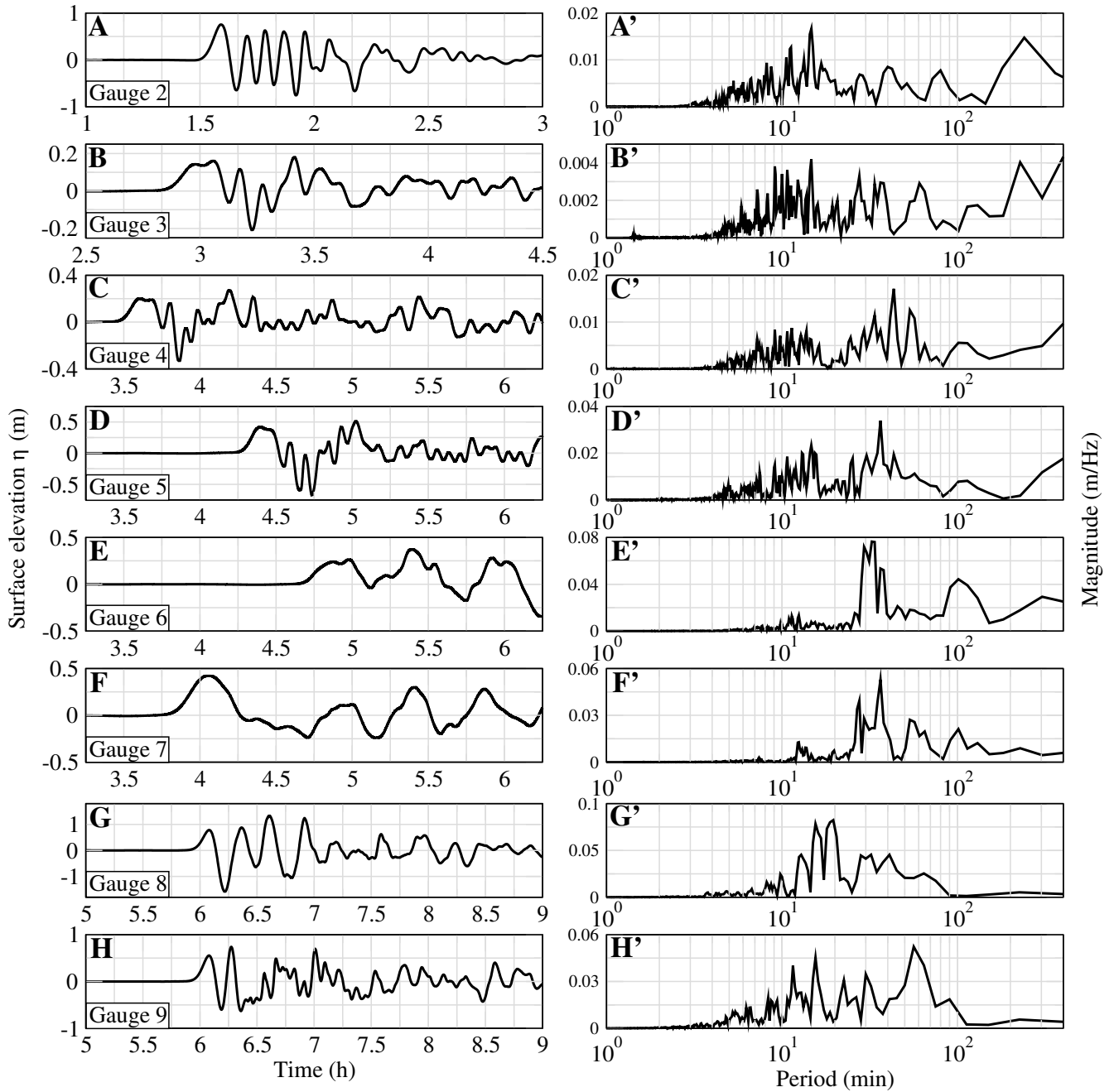
Figure 17. Surface elevations (m) (left column) and Fourier transforms (right column) for the 80 \text{ km}^3 scenario at Gauge 2 in south Portugal (A and A'), Gauge 3 in the abyssal plain of the Bay of Biscay (B and B'), Gauge 4 in the continental shelf of the Bay of Biscay (C and C'), Gauge 5 in south Brittany (D and D'), Gauge 6 in the Gironde estuary (E and E'), Gauge 7 in Saint-Jean-de-Luz (F and F') and Gauges 8 and 9, respectively north (G and G') and south (H and H') of Guadeloupe, computed by FUNWAVE-TVD. The time takes into account the 20 first minutes of the slide and tsunami generation.
