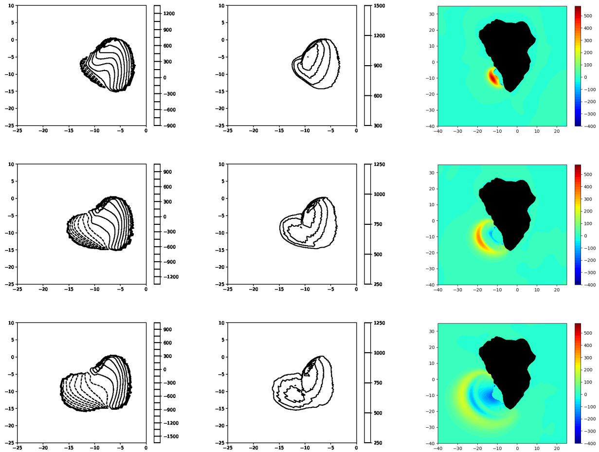
Figure 9. Snapshots of slide upper free surface, thickness and corresponding water free surface for the present study ( i.e. , viscous slide with a viscosity of 2 \times 10^7 Pa-s, (left, middle, right) respectively) for the 80 \text{ km}^3 scenario at t=60 s (row 1), 120 s (row 2), 180 s (row 3).
