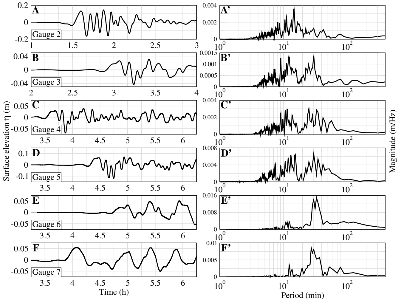
Figure 18. Surface elevations (m) (left column) and Fourier transforms (right column) for the 20 \text{ km}^3 scenario at Gauge 2 in south Portugal (A and A'), Gauge 3 in the abyssal plain of the Bay of Biscay (B and B'), Gauge 4 in the continental shelf of the Bay of Biscay (C and C'), Gauge 5 in south Brittany (D and D'), Gauge 6 in the Gironde estuary (E and E') and Gauge 7 in Saint-Jean-de-Luz (F and F'), computed by FUNWAVE-TVD. The time takes into account the 20 first minutes of the slide and tsunami generation.
