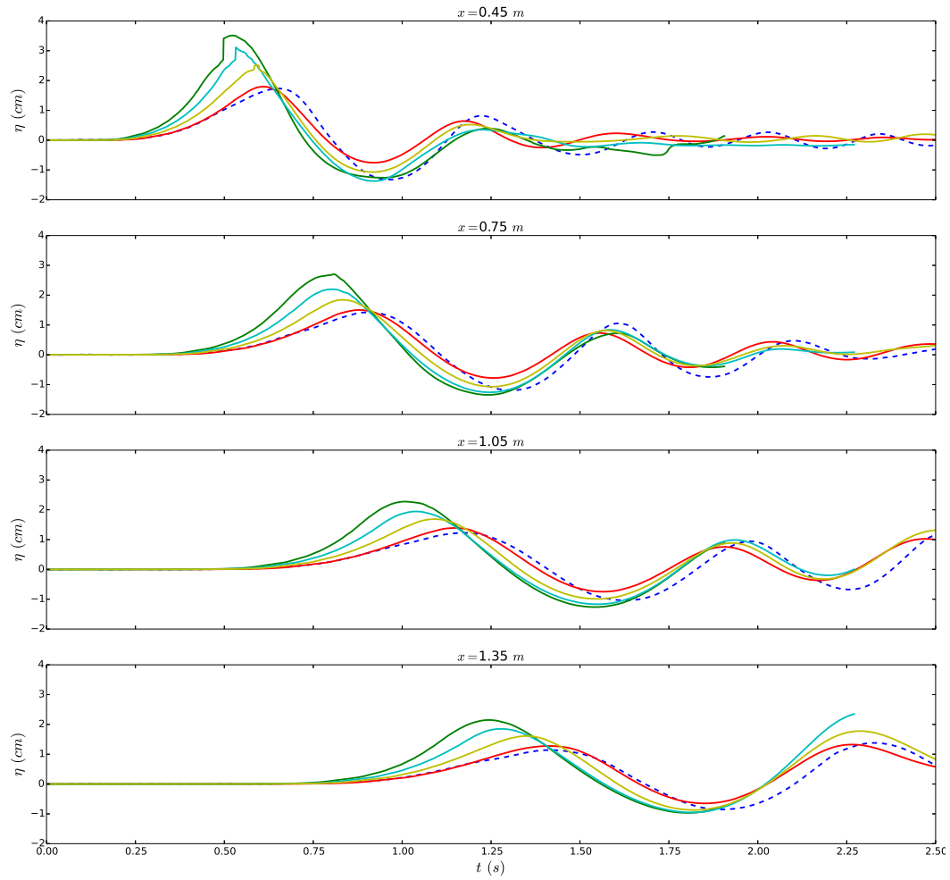
Figure 3. Free-surface elevation at the gauges for the experiment (blue dashed line) and the simulations for different values of viscosity, \mu=1 \text{ Pa}\cdot\text{s} : green line, \mu=2 \text{ Pa}\cdot\text{s} : cyan line, \mu=5 \text{ Pa}\cdot\text{s} : yellow line and \mu=10 \text{ Pa}\cdot\text{s} : red line.
