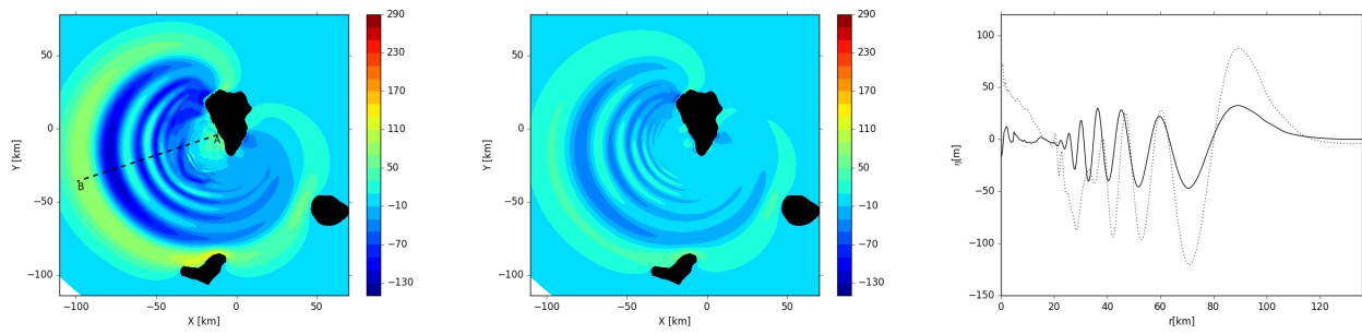
Figure 12. THETIS 3D computations for the 80 \text{ km}^3 slide scenario, t \approx 560 \text{ s} . left panel: Inviscid slide. middle panel: Slide viscosity 2 \times 10^7 \text{ Pa}\cdot\text{s} . right panel: Free surface elevations along the cross section A-B (left panel).
