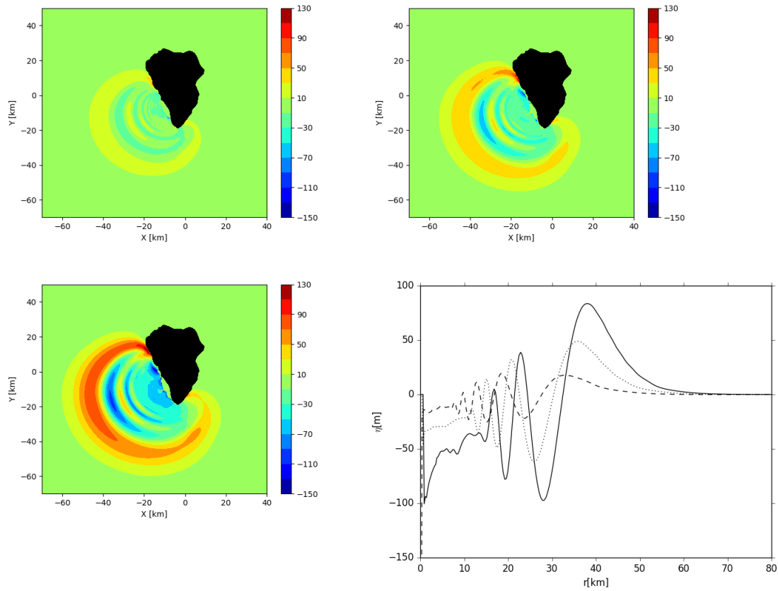
Figure 13. THETIS 3D computations for : 20 \text{ km}^3 (top, left), 40 \text{ km}^3 (top, right) and 80 \text{ km}^3 (bottom, left) slide scenarios at t=5 \text{ min} . Bottom right panel: Free surface elevations along section A-B of left frame of Figure 12. Slide viscosity 2 \times 10^7 \text{ Pa}\cdot\text{s} .
