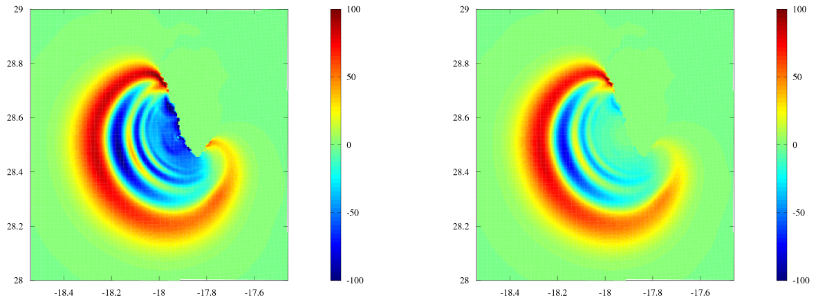
Figure 14. Region around Cumbre Vieja Volcano after 5 minutes of simulated time with THETIS for the 80 \text{ km}^3 slide scenario. Left : Wave elevation for the initial solution from THETIS. Right : Filtered state which is used to initialize FUNWAVE-TVD.
