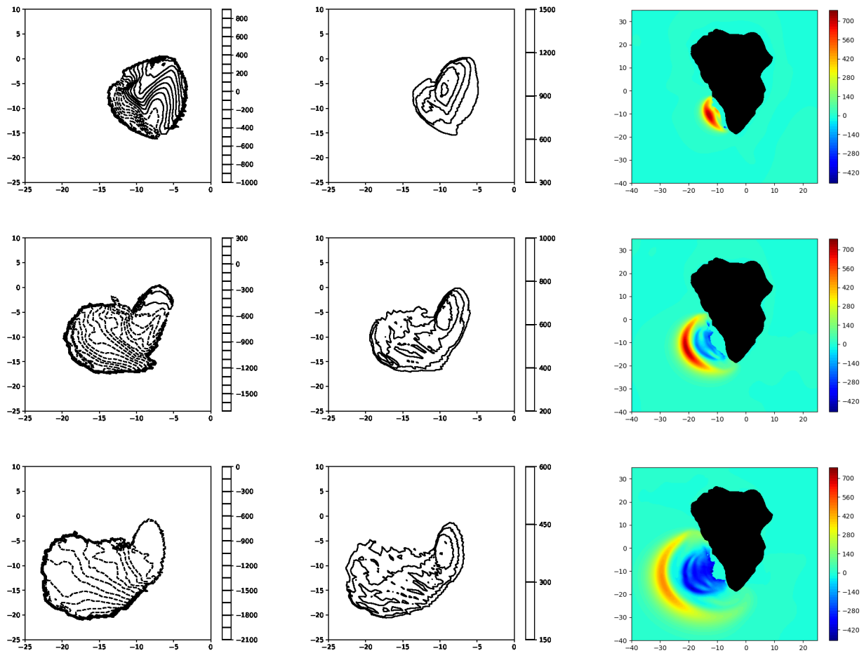
Figure 8. Snapshots of slide upper free surface, thickness and corresponding water free surface for the inviscid case (Abadie et al., 2012) (left, middle, right) respectively) for the 80 \text{ km}^3 scenario at t=60 \text{ s} (row 1), 120 \text{ s} (row 2), 180 \text{ s} (row 3).
