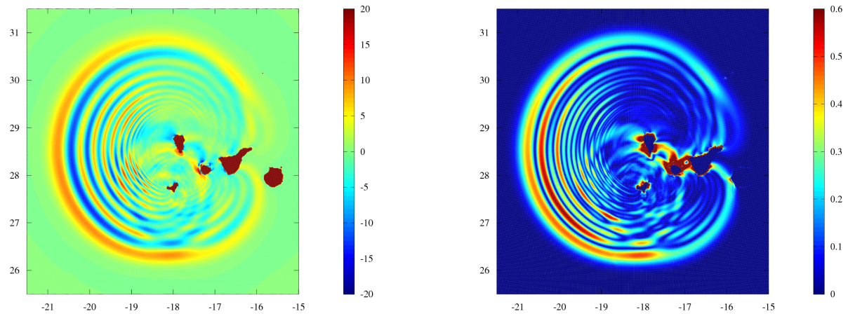
Figure 16. Region around the Canary Islands, 20 minutes after the beginning of the event (after 5 minutes of simulated time with THETIS, and 15 minutes of simulated time with FUNWAVE-TVD) during the 80 \text{ km}^3 slide volume scenario. Left: Wave elevation. Right: Horizontal water velocity magnitude.
