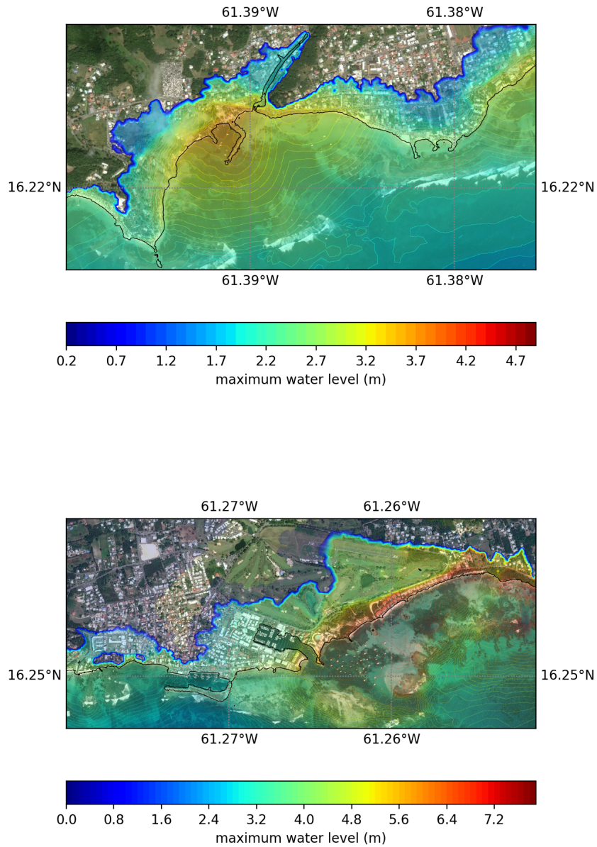
Figure 23. Flood map showing the maximum water level reached during the 80 km 3 scenario for the region of Sainte-Anne (top) and Saint-François (bottom) (see locations in Figure 7), computed by SCHISM. Map created using ArcGIS® software by Esri. ArcGIS® and ArcMap™ are the intellectual property of Esri and are used herein under license. Copyright © Esri. All rights reserved.
