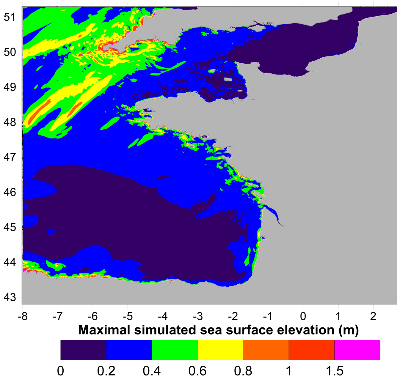
Figure 21. Maximum surface elevations (m) computed by FUNWAVE-TVD for the 80 km 3 scenario on the western French coasts, with a 450-m resolution.
