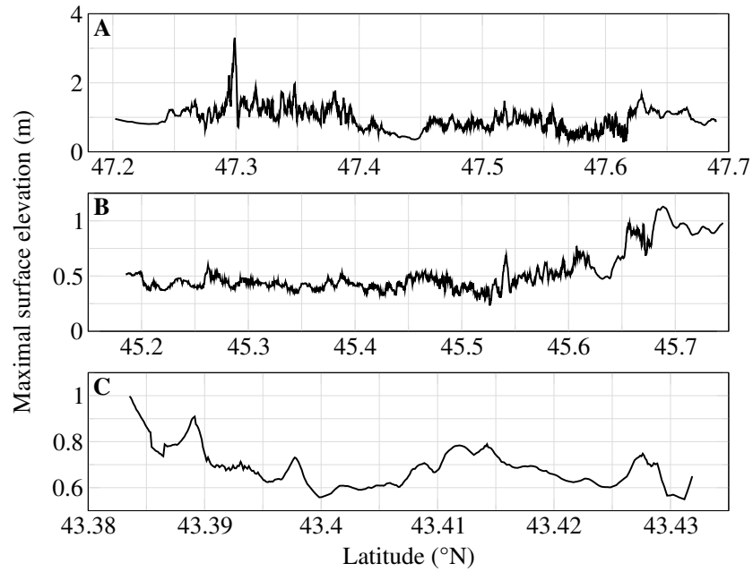
Figure 22. Maximum surface elevation computed with Calypso for the 80 km 3 scenario using the finest grid resolution at isobath -5 m for different areas along the French Atlantic coastline. Panel A: Morbihan, panel B: Gironde estuary, panel C: Saint-Jean-de-Luz area
