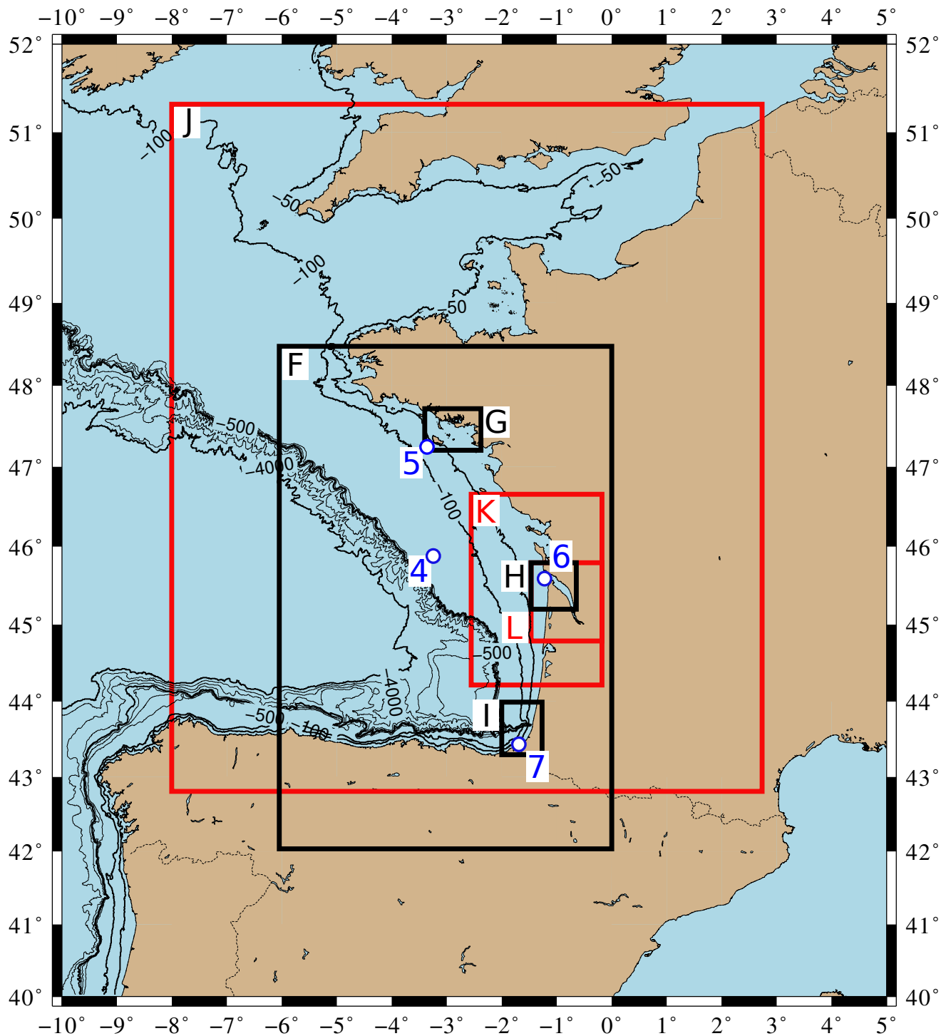
Figure 5. Computational domains for Calypso (500-m resolution (F), 125 m (G) or 32.5 m (H and I) in black) and FUNWAVE-TVD (450 m (J), 110 m (K) and 20 m (L) in red). After the -50 m contour, bathymetric contours range from -100 m to -500 m every 100 m, then from -1000 m to -4000 m every 1000 m. Gauges 4, 5, 6 and 7 are marked by the white and blue points.
