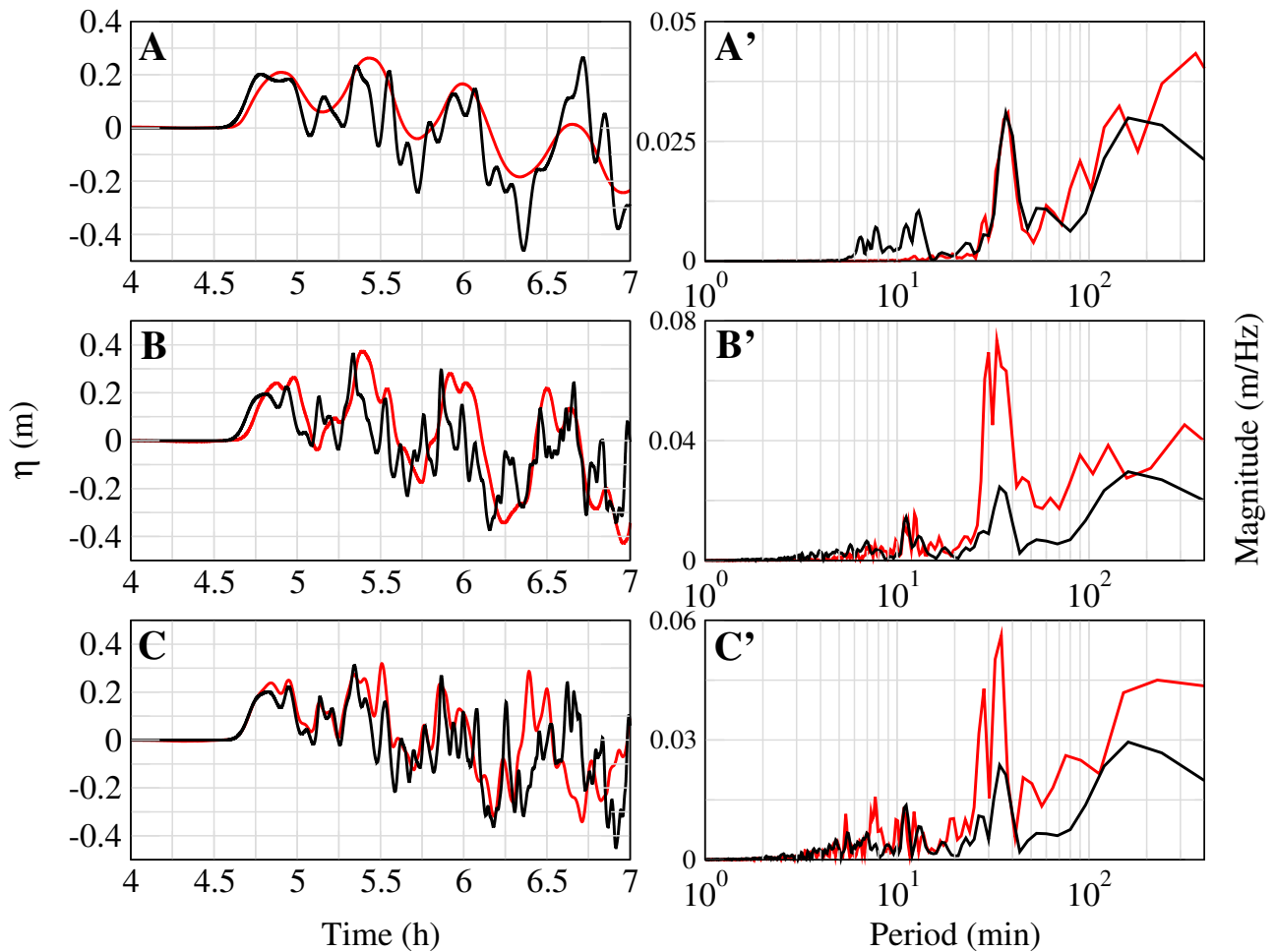
Figure 19. Comparison of the surface elevation (m) and the associated periods computed by a Fourier transformation (A', B' and C') at Gauge 6 between Calypso (in black) and FUNWAVE-TVD (in red) for the 80 \text{ km}^3 scenario at the Gironde estuary, for three resolutions: 2.7 km (A), 450 m (B) and 110 m (C) for FUNWAVE-TVD and 2 km (A), 500 m (B) and 125 m (C) for Calypso. The time takes into account the 20 first minutes of the slide and tsunami generation.
