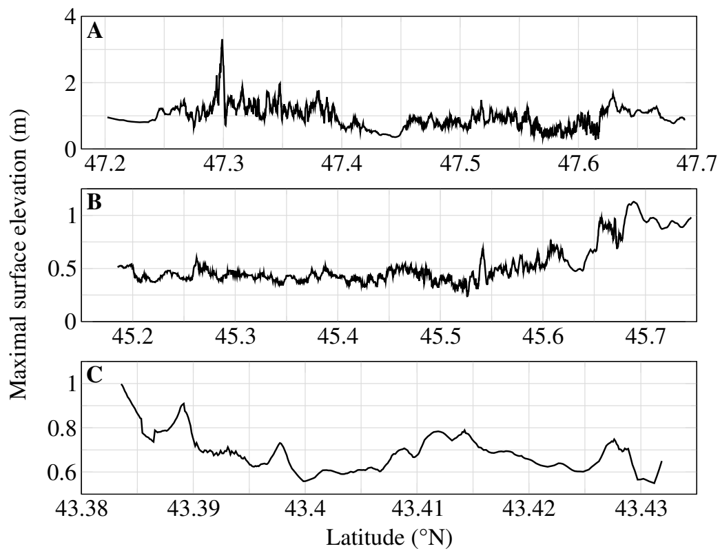
Figure 22. Maximum surface elevation computed with Calypso for the 80 \text{ km}^3 scenario using the finest grid resolution at isobath -5 m for different areas along the French Atlantic coastline. Panel A: Morbihan, panel B: Gironde estuary, panel C: Saint-Jean-de-Luz area
