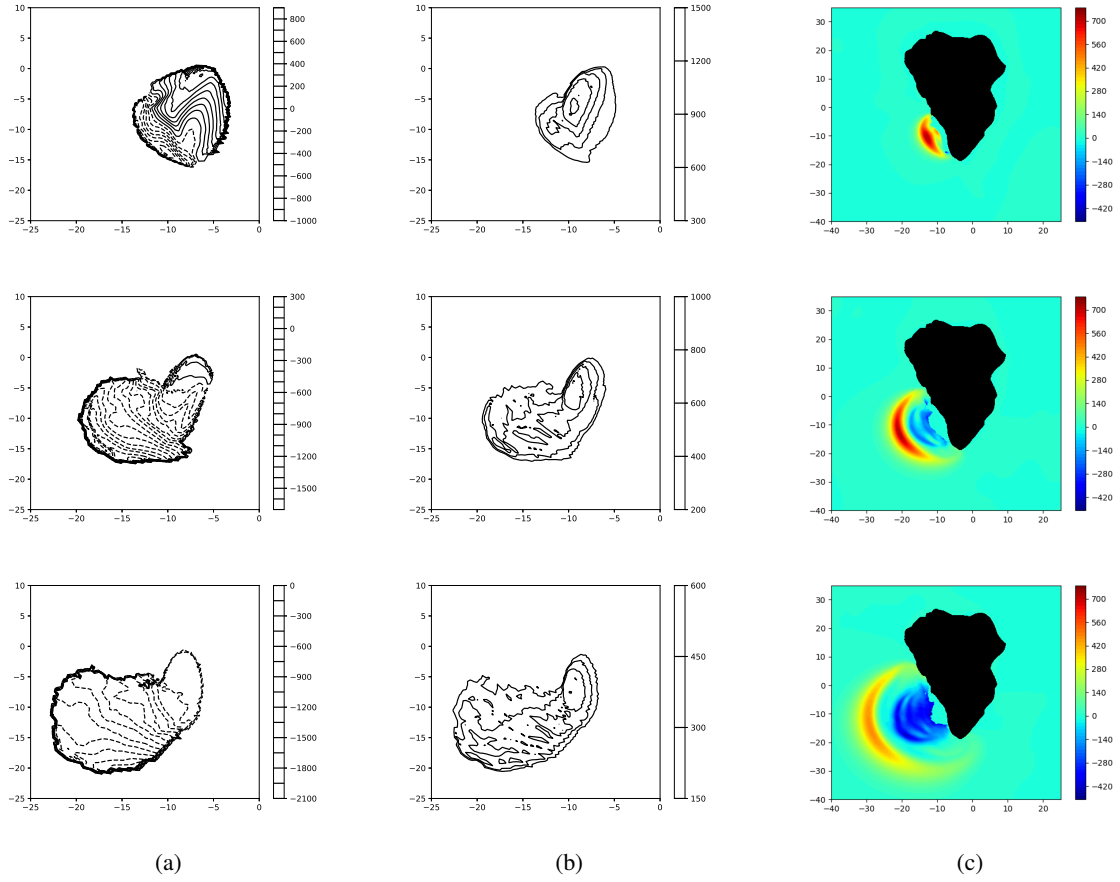
Figure 8. Snapshots of slide upper free surface, thickness and corresponding water free surface for the inviscid case (Abadie et al., 2012) ((a), (b), (c)) respectively) for the 80 \text{ km}^3 scenario at t=60 \text{ s} (row 1), 120 \text{ s} (row 2), 180 \text{ s} (row 3).
