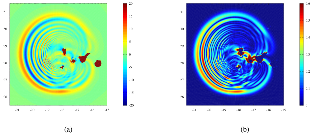
Figure 16. Region around the Canary Islands, 20 minutes after the beginning of the event (after 5 minutes of simulated time with THETIS, and 15 minutes of simulated time with FUNWAVE-TVD) during the 80 \text{ km}^3 slide volume scenario. (a): Wave elevation. (b): Horizontal water velocity magnitude.
