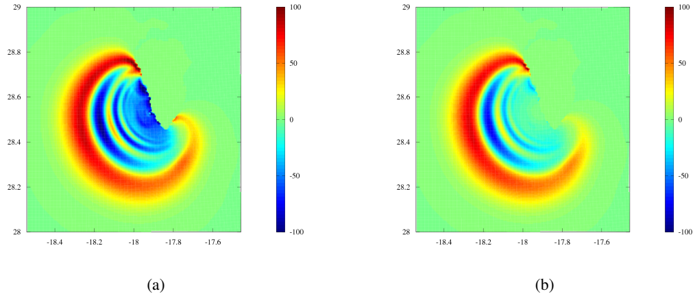
Figure 14. Region around Cumbre Vieja Volcano after 5 minutes of simulated time with THETIS for the 80 km 3 slide scenario. (a): Wave elevation for the initial solution from THETIS. (b): Filtered state which is used to initialize FUNWAVE-TVD.
