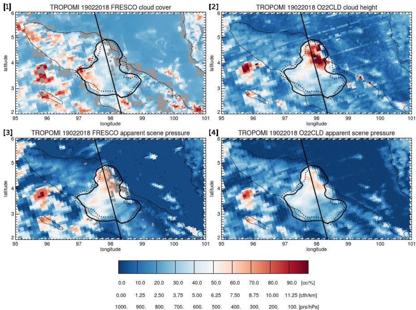
Figure 1B. As figure 1A but for TROPOMI FRESCO cloud cover (panel [1]), O22CLD cloud height (panel [2]), FRESCO 490 apparent scene pressure (panel [3]) and O22CLD apparent scene pressure (panel [4]).
