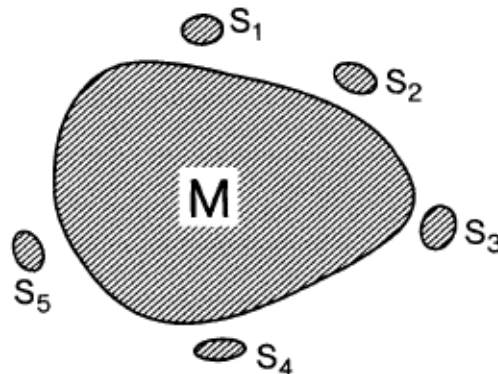
Figure 2. Schematic diagram for Model II. The shaded area M denotes the main-shock slip zone. The smaller cracks S_j , denote small satellite faults that surround the main-shock fault. The gaps between the satellites and the edge of the main shock fracture disappear by stress corrosion.
