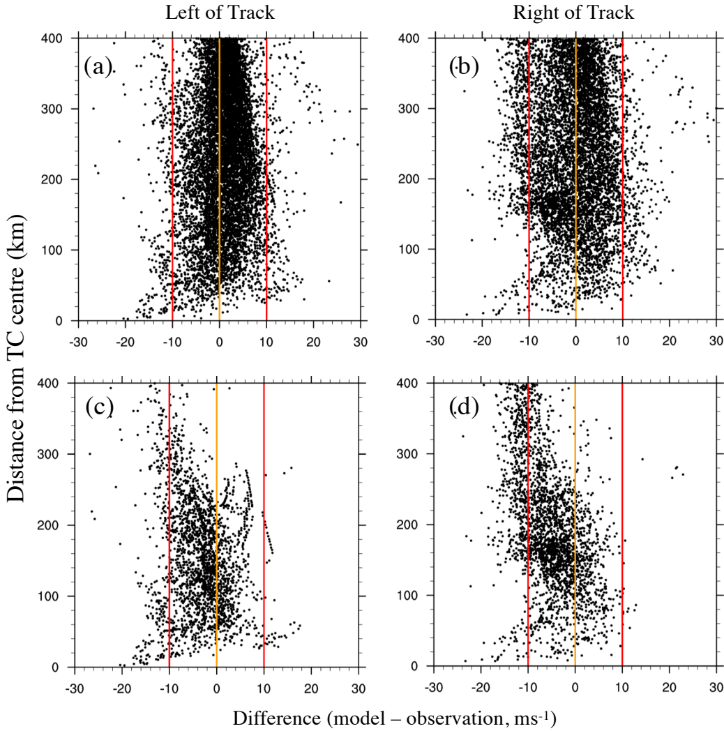
Figure 4: Difference between modelled and observed wind speeds for the 8 U.S. storms as a function of distance from the TC centre (ms -1 ) and split by left of track (left column) and right of track (right column). The upper row shows all data points, and the lower row shows only urban data points that experienced observed wind speeds greater than 18 ms -1 . The orange lines indicate zero difference and the red lines indicate a positive and negative difference of 10 ms -1 .
