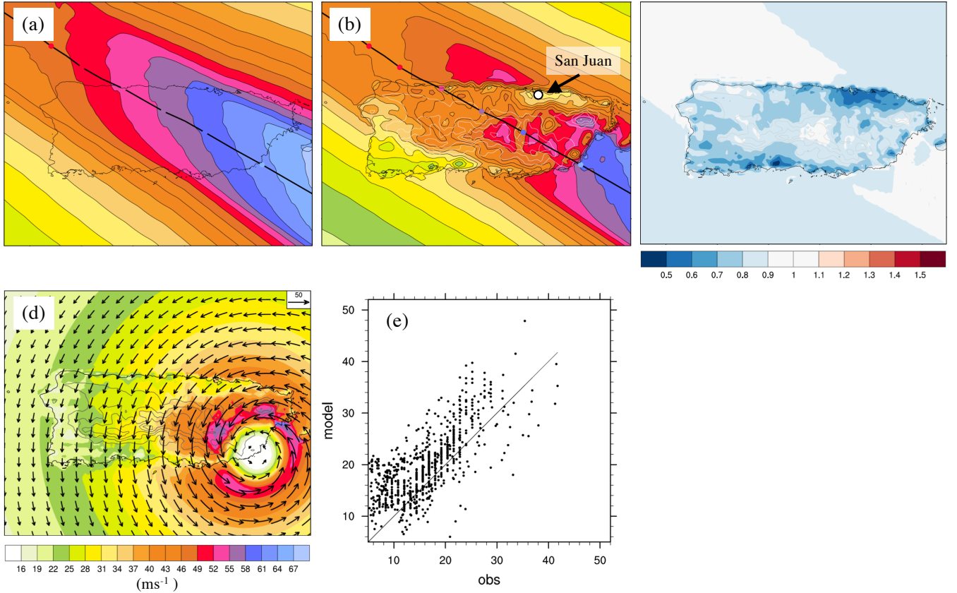
Figure 2: Case study simulation of Hurricane Maria (2017) over Puerto Rico. Simulated footprints ( \text{ms}^{-1} ) are shown using (a) Willoughby only, (b) Willoughby and KW01. The hurricane track is shown by the thick black line with input V_{\text{max}} shown every six hours along the track (coloured dots). Coastlines are shown by the thin black lines, and are only included in (a) to aid interpretation. (c) The ratio of Willoughby and KW01 to Willoughby only. (d) A snapshot of the simulation using Willoughby and KW01 at the time of landfall (wind speed is contoured and wind vectors are shown in arrows). Terrain height is contoured every 200 m in (b) – (d). (e) A comparison of observed and simulated (Willoughby and KW01) winds.
