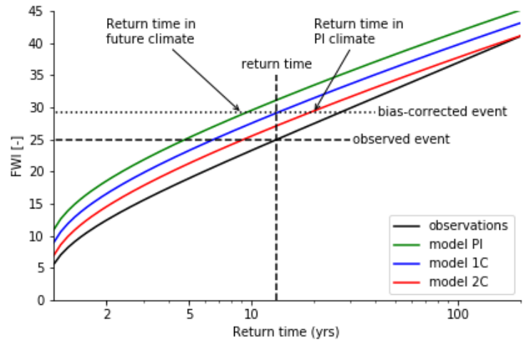
505 Figure 3: Schematic of the bias correction method.
