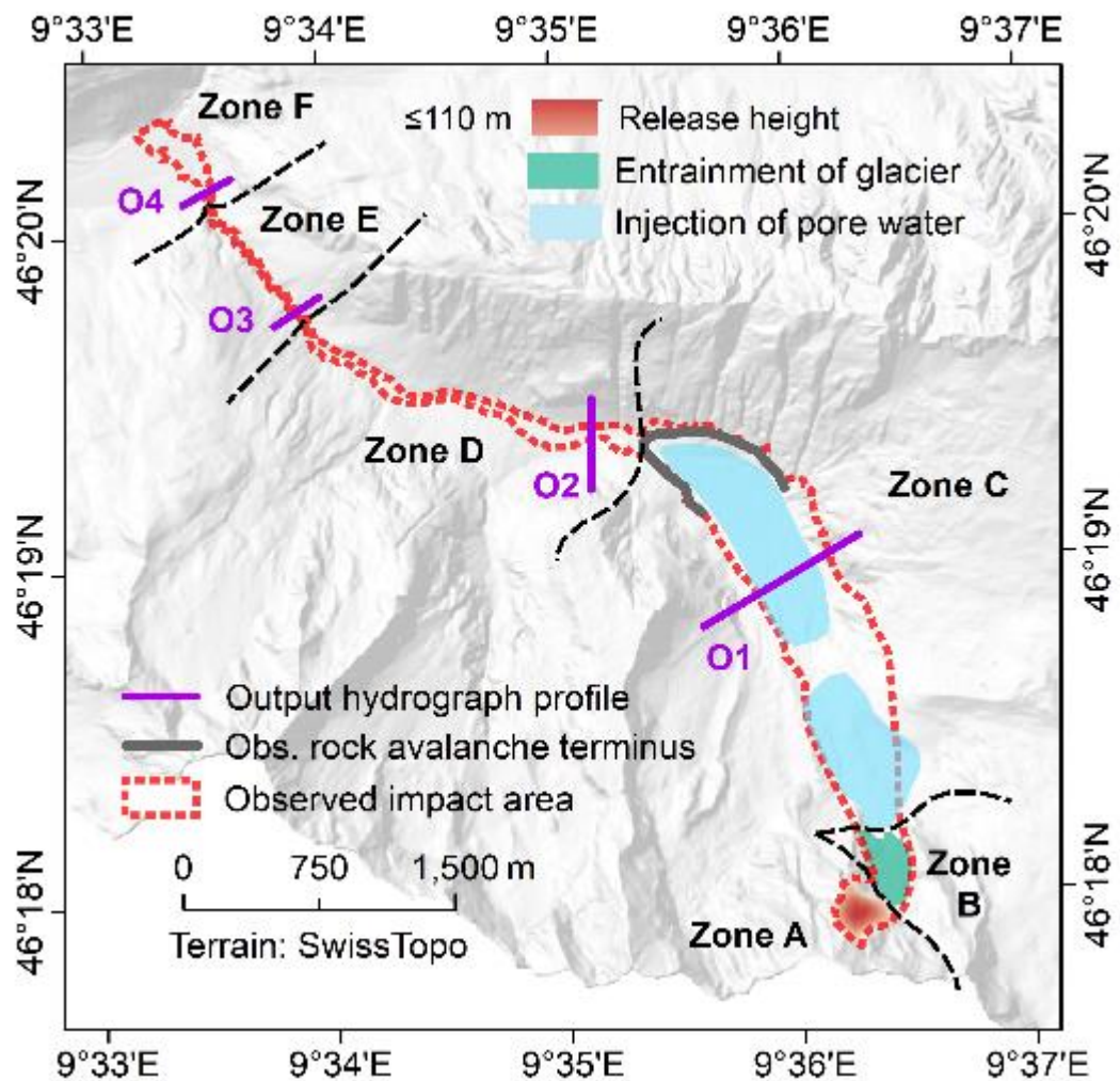
Figure 7. Overview of the heights and entrainment areas as well as the zonation performed as the basis for the simulation with r.avaflo. Injection of pore water only applies to the Scenario A. The zones A–F represent areas with largely homogeneous surface characteristics. The characteristics of the zones and the model parameters associated to each zone are summarized in Table 1 and Fig. 4. O1–O4 represent the output hydrograph profiles. The observed rock avalanche terminus was derived from WSL (2017).
