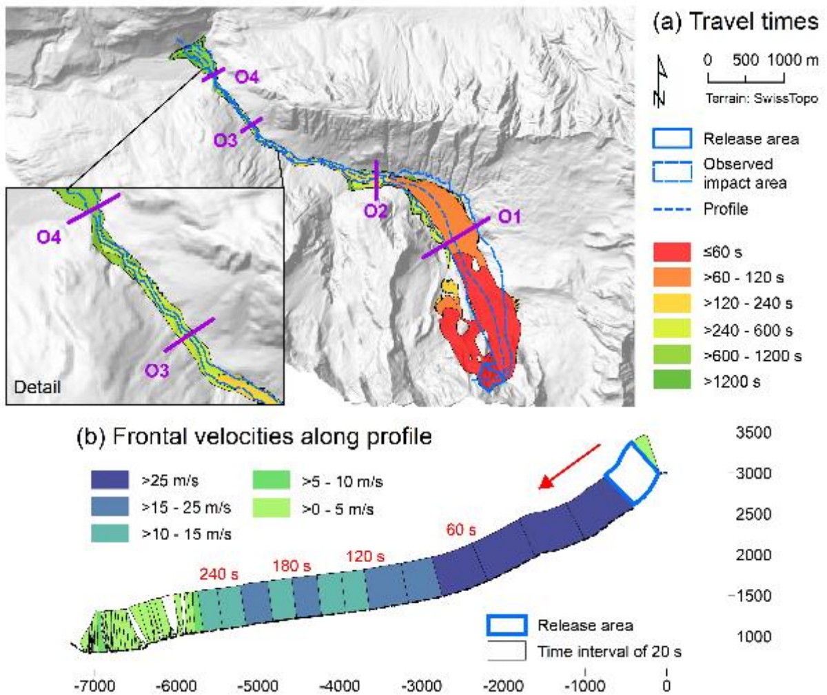
Figure 10. Spatio-temporal evolution and velocities of the event obtained for Scenario S1 . (a) Travel times, starting from the release of the initial rock slide-rock fall. (b) Frontal velocities along the flow path, shown in steps of 20 s. Note that the height of the velocity graph does not scale with flow height. White areas indicate that there is no clear flow path.
