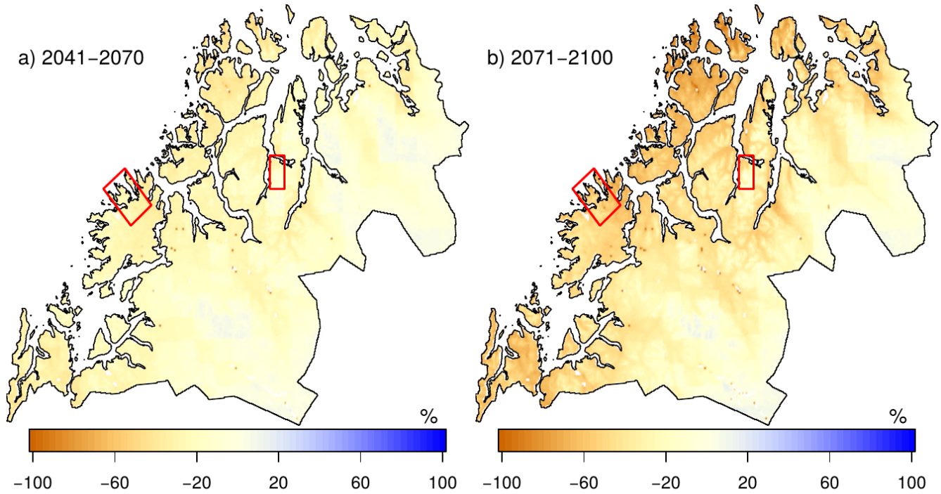
5 Figure 9: Projected change in maximum 1-day snowfall during winter (Oct–Apr) between 1981–2010 and a) near future (2041–2070); b) far future (2071–2100, based on maximum fresh snow water equivalent for 1-day duration (WM-FSW-1d).
