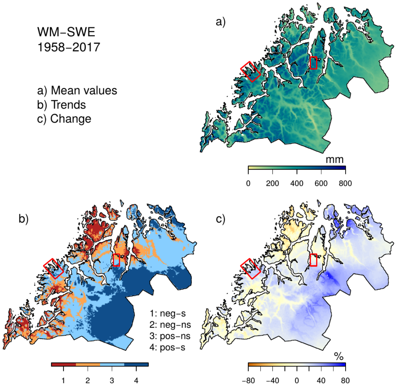
5 Figure 4: Mean values (a), trends (b) and changes (c) in winter (Oct-Apr) maximum snow water equivalent (SWE) for the period 1958–2017. In b), positive trends are illustrated in blue and negative trends in red; dark red and blue colors represent statistically negative and positive significant (s) trends, respectively. Light colors represent statistically not-significant (ns) trends. In c), percentage changes between the two 30-year periods 1958–1987 and 1988–2017 are shown.
