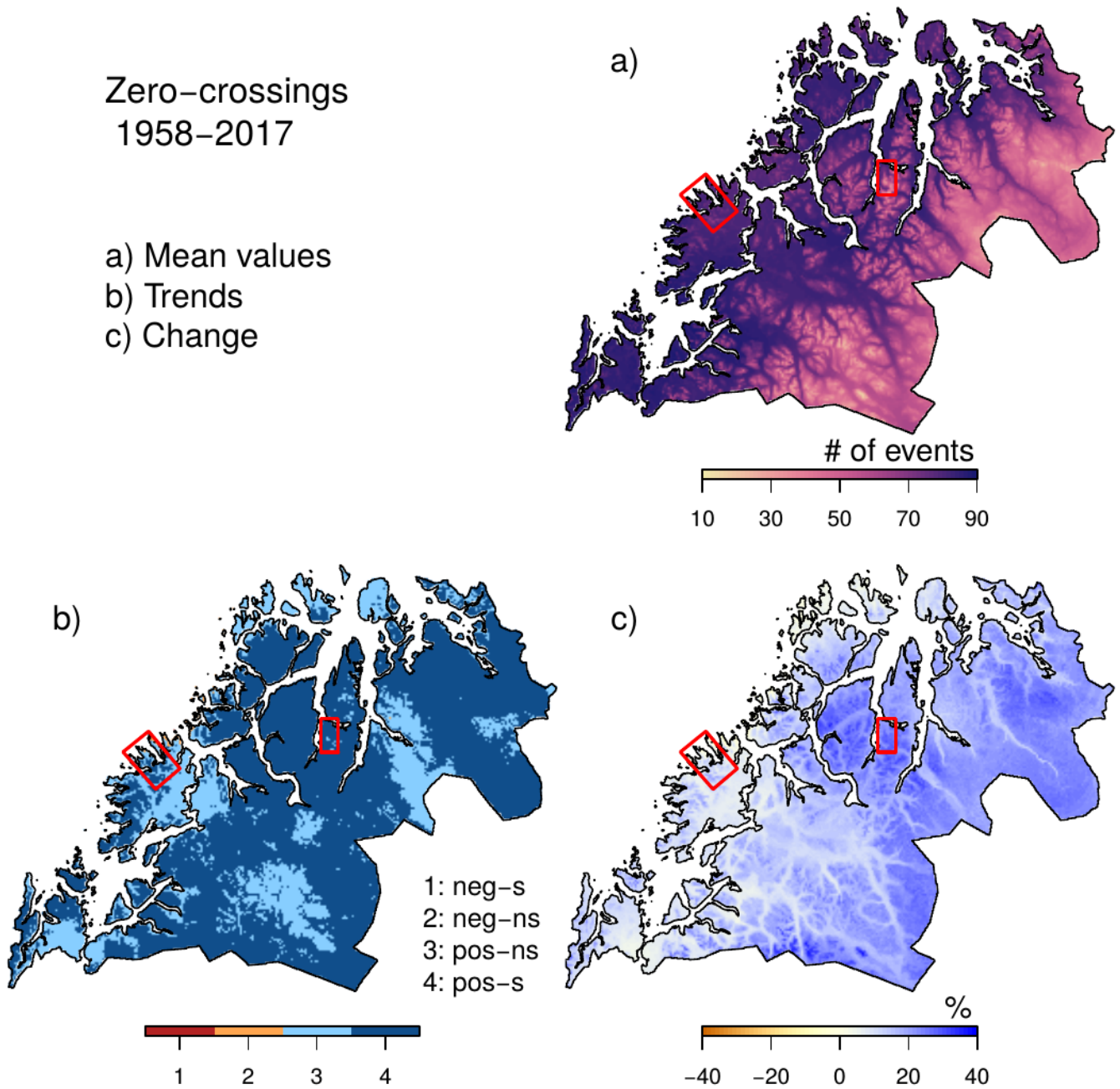
Figure 12: Frequency of zero-crossings during winter (Oct–Apr) for the period 1958–2017, based on minimum and maximum daily temperature. Mean values (a), trends (b) and changes are shown in the same way as in Fig. 4.
