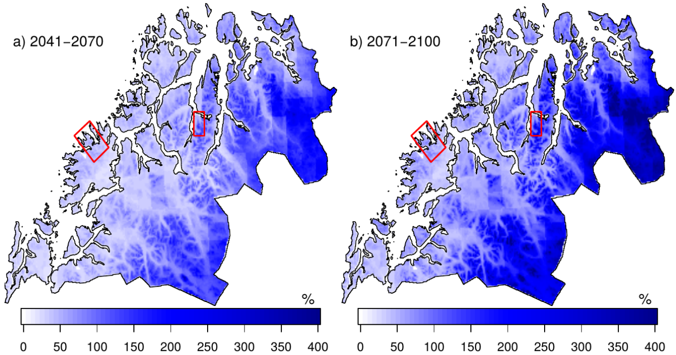
5 Figure 15: Projected change in the frequency of rainfall events exceeding 10 mm during winter (Oct–Apr) between 1981–2010 and a) near future (2041–2070) and b) far future (2071–2100). Note that the legend differs from other figures, going from 0 to 400 %.
