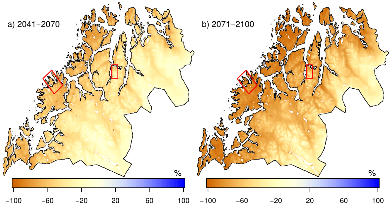
Figure 11: Projected change in the frequency of 1-day snowfall exceeding 5 mm during winter (Oct–Apr) between 1981–2010 and a) near future (2041–2070) and b) far future (2071–2100), based on fresh snow water equivalent for 1-day duration (FSW-1d > 5 mm).
