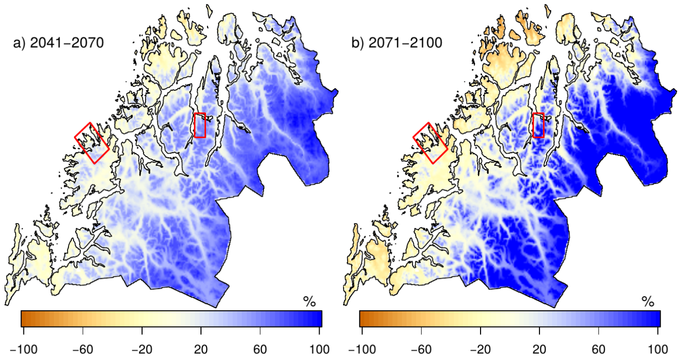
Figure 13: Projected change in the frequency of zero-crossings during winter (Oct–Apr) between 1981–2010 and a) near future (2041–2070) and b) far future (2071–2100), based on minimum and maximum temperature.
