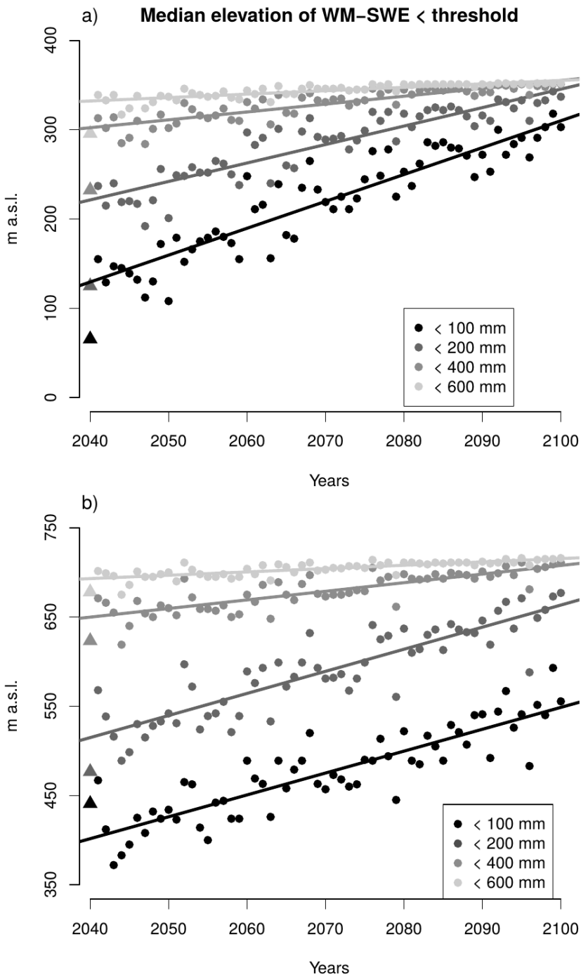
Figure 7: Projected future development in median elevation where winter maximum SWE is below 100 mm (black), 200 mm (dark grey), 400 mm (medium grey) or 600 mm (light grey). a) Coast and b) inland (see map in Fig. 1). Mean values for the period 1981–2010 are indicated as triangles.
