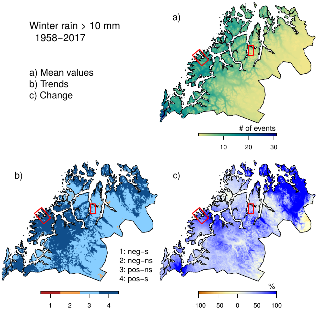
Figure 14: Frequency of rainfall events exceeding 10 mm during winter (Oct–Apr) for the period 1958–2017, based on minimum and maximum daily temperature. Mean values (a), trends (b) and changes are shown in the same way as in Fig. 4.
