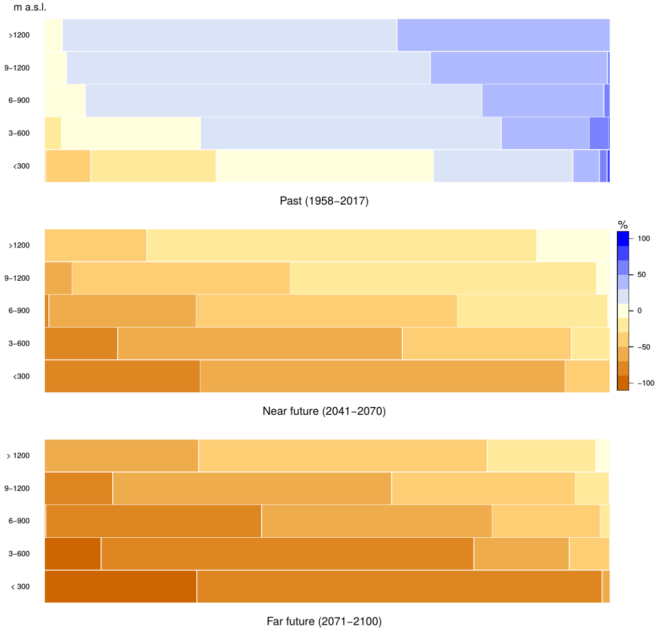
5 Figure 6: Percentage change in winter maximum SWE in different elevation levels for: historical period (change between 1958–1987 and 1988–2017; upper panel), near future (change between 1981–2010 and 2041–2070; middle panel) and far future (change between 1981–2010 and 2071–2100; lower panel). The length of the colored bars represent the fraction of grid cells within the different intervals of change given by the legend.
