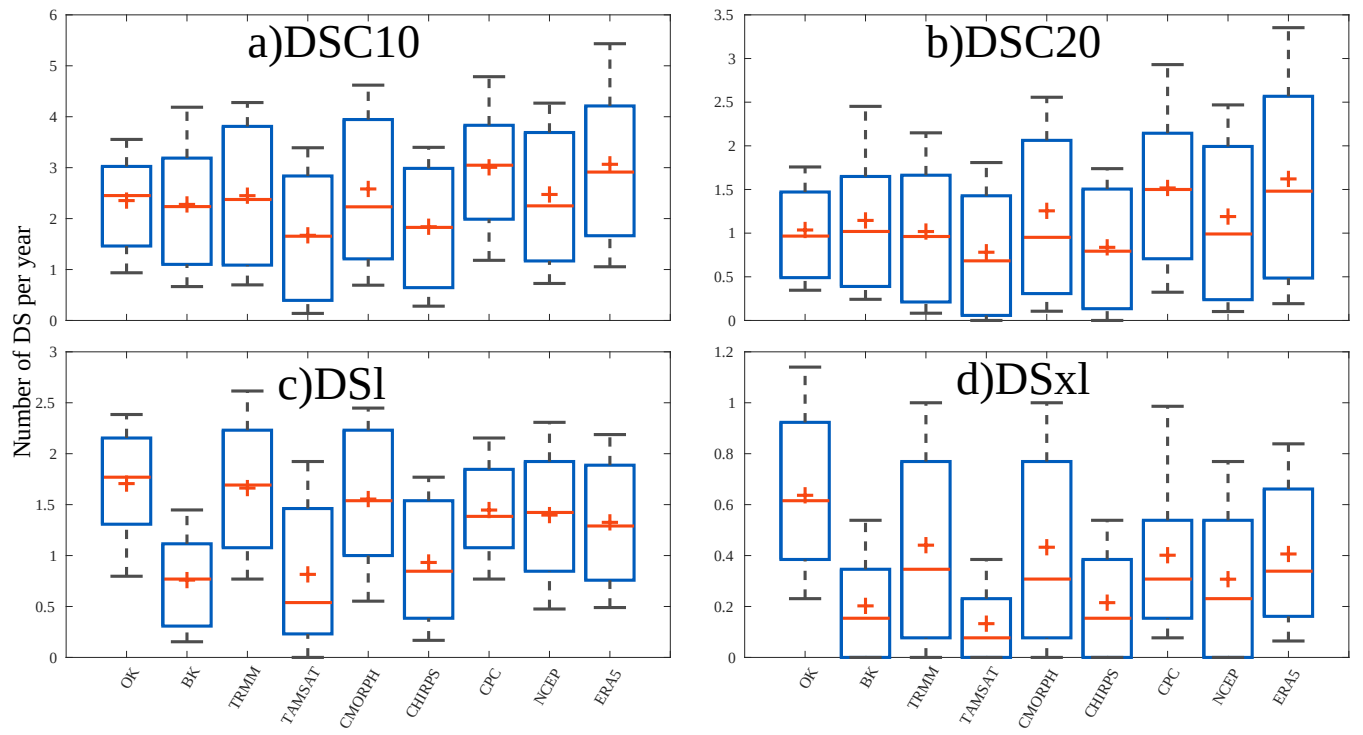
Figure 6. Box plots of average number of dry spells (DSC10, DSC20, DSI and DSxl) per year collected on all grid points for the 9 gridded datasets used ( TRMM, TAMSAT, CMORPH, CHIRPS, CPC, NCEP, ERA5, BK, OK). The minus sign (-) represents the median value, the plus sign (+) represents the mean value, the bottom and top edges of the box represent the 25th and 75th percentile values, respectively, while the “whiskers” represent the extreme values (5 and 95%). The average number of dry spells is computed on the overlap period (1998-2010). Details on the datasets and dry spells are provided in Tables 1 and 2, respectively.
