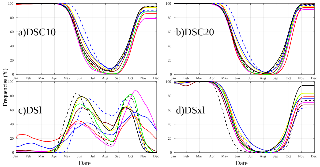
Figure 7. Seasonal cycle of four categories of dry spells (DSC10, DSC20, DSI and DSxl) used in this study computed on the overlap between datasets (1998-2010): TRMM, TAMSAT, CMORPH, CHIRPS, CPC, NCEP, ERA5, BK, OK. Frequency is defined as a ratio of observational days with recorded dry spells. Details on the datasets and dry spells are provided in Tables 1 and 2, respectively.
