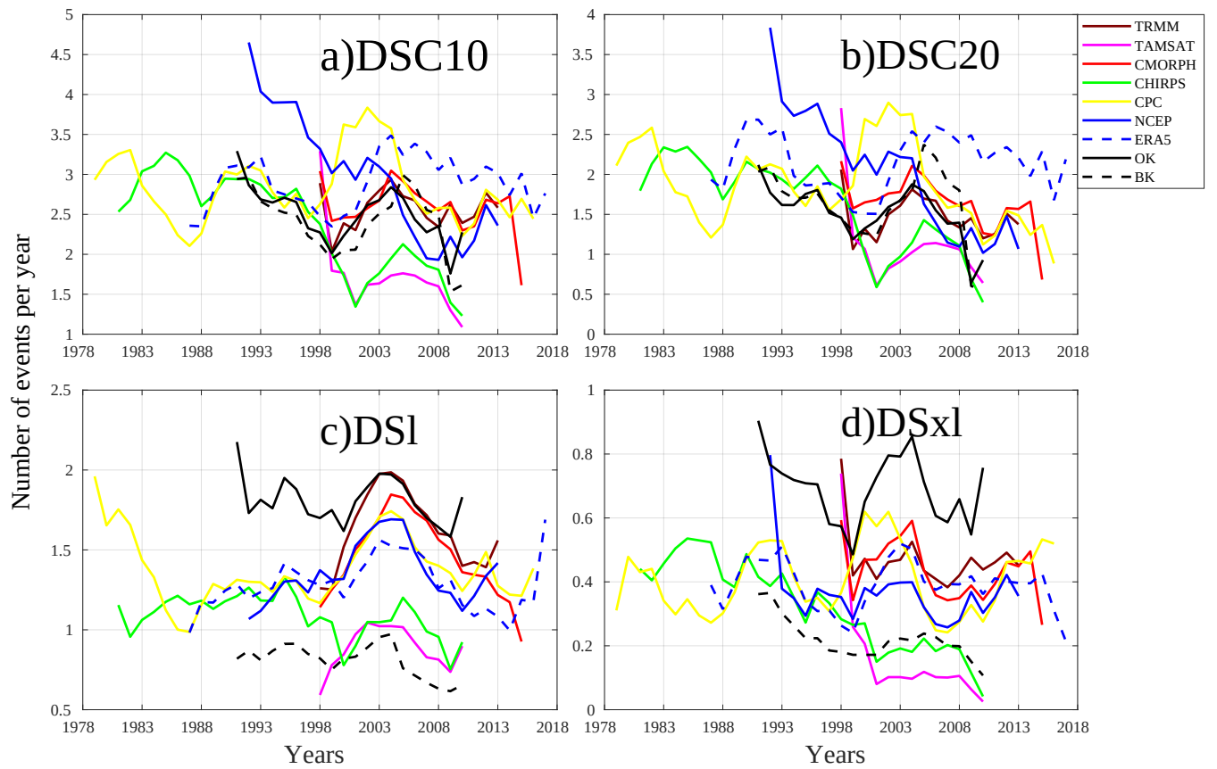
Figure 9. Interannual variability of average numbers on all grid points of DSC10, DSC20, DSI and DSxl computed over the period of availability for each dataset: TRMM (1998-2013), TAMSAT(1998-2010), CMORPH (1998-2015), CHIRPS (1981-2010), CPC (1979-2016), NCEP (1992-2013), ERA5 (1987-2017), BK (1991-2010), OK (1991-2010). Details on the datasets and dry spells are provided in Tables 1 and 2, respectively.
