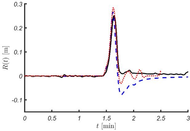
160 Figure 3: Run-up height of the long single wave with A = 0.1 m and T = 20 s on a beach slope \tan \alpha = 1:6 , the numerical solution is shown with the red dots line, analytical solution is shown with blue dashed line and the experimental record is shown with the black solid line.
