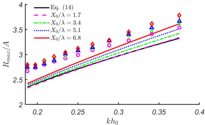
210 Figure 6: Maximum run-up height, R_{\max}/A as a function of kh_0 for different distances to the slope, X_0/\lambda . Analytical solution described in Section 2 is shown with lines and numerical solution described in Section 3 is shown with symbols (diamonds, triangles, squares and circles) with matching colours. The thick black line corresponds to Eq. (14) for wave run-up on a beach without constant depth section, A/h_0 = 0.03 .
