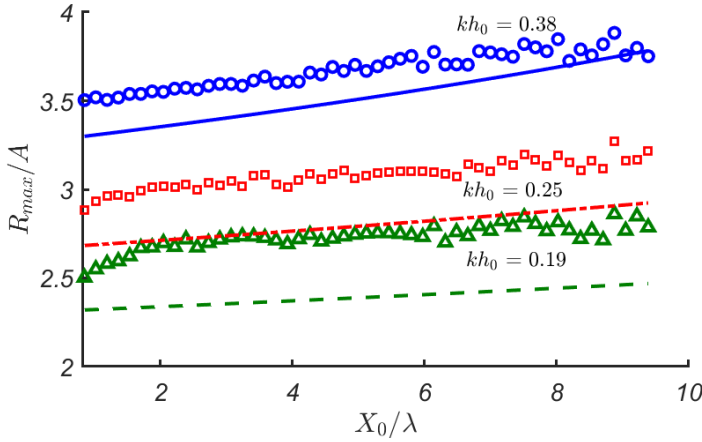
245 Figure 8: Maximum run-up height, R_{\max}/A as a function of the distance to the slope, X_0/\lambda for different kh_0 . Analytical solution described in Section 2 is shown with lines and numerical solution described in Section 3 is shown with symbols (triangles, squares and circles) with matching colours; A/h_0 = 0.03 .
