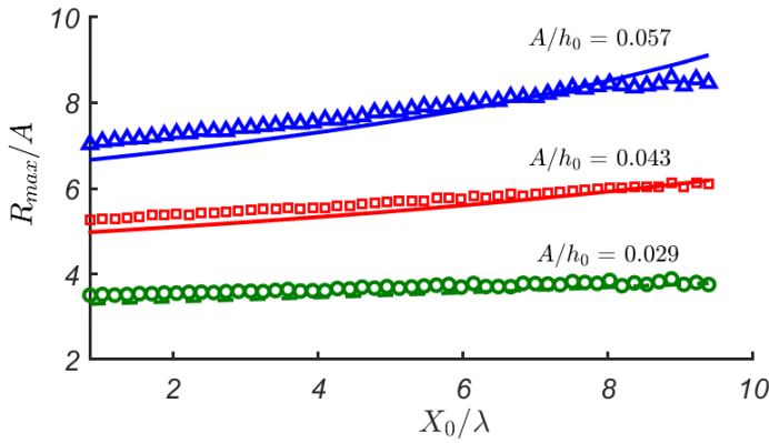
Figure 5: Maximum run-up height, R_{\max}/A , as a function of distance to the slope, X_0/\lambda for different amplitudes of the initial wave, A/h_0 . Analytical solution described in Section 2 is shown with lines and numerical solution described in Section 3 is shown with symbols (triangles, squares and circles) with matching colours, kh_0 = 0.38 .
