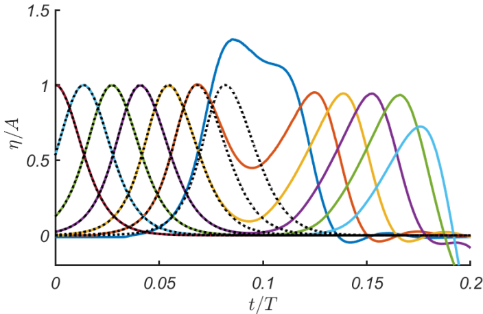
255 Figure 9: Wave evolution at different locations x/\lambda = 0, 0.85, 1.71, 2.56, 3.41, 4.27 and 5.12 along the section of constant depth for a basin with X_0/\lambda = 5.12 and \tan \alpha = 1:20 . Numerical results are shown with solid lines, while the analytical predictions are given by the black dotted lines. The parameters of the wave: A/h_0 = 0.03, kh_0 = 0.19 .
