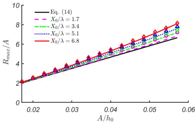
Figure 4: Maximum run-up height, R_{\max}/A , as a function of initial wave amplitude, A/h_0 , for different distances to the slope, X_0/\lambda . Analytical solution described in Section 2 is shown with lines and numerical solution described in Section 3 is shown with symbols (diamonds, triangles, squares and circles) with matching colours. The thick black line corresponds to Eq. (14) for wave run-up on a beach without constant depth section, kh_0 = 0.38 .
