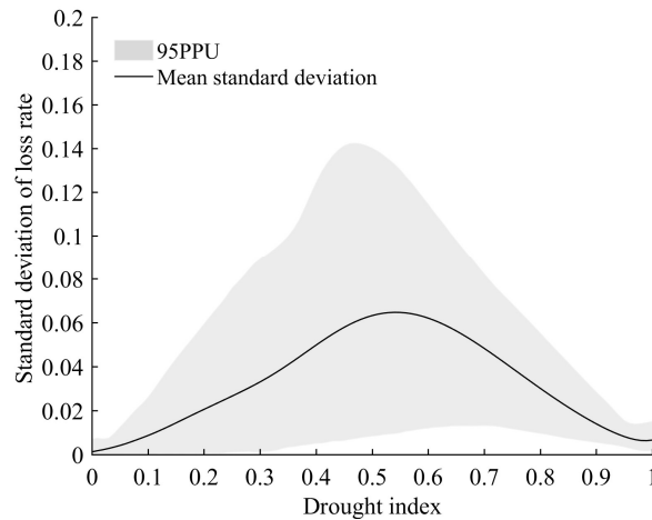
Figure 9: Distribution of standard deviation of loss rate under different drought index. The mean standard deviation and 95 % prediction uncertainty band (95PPU) are calculated by the standard deviations of sample grids, which are randomly selected from the five vulnerability curves at a proportion of 10 %.
