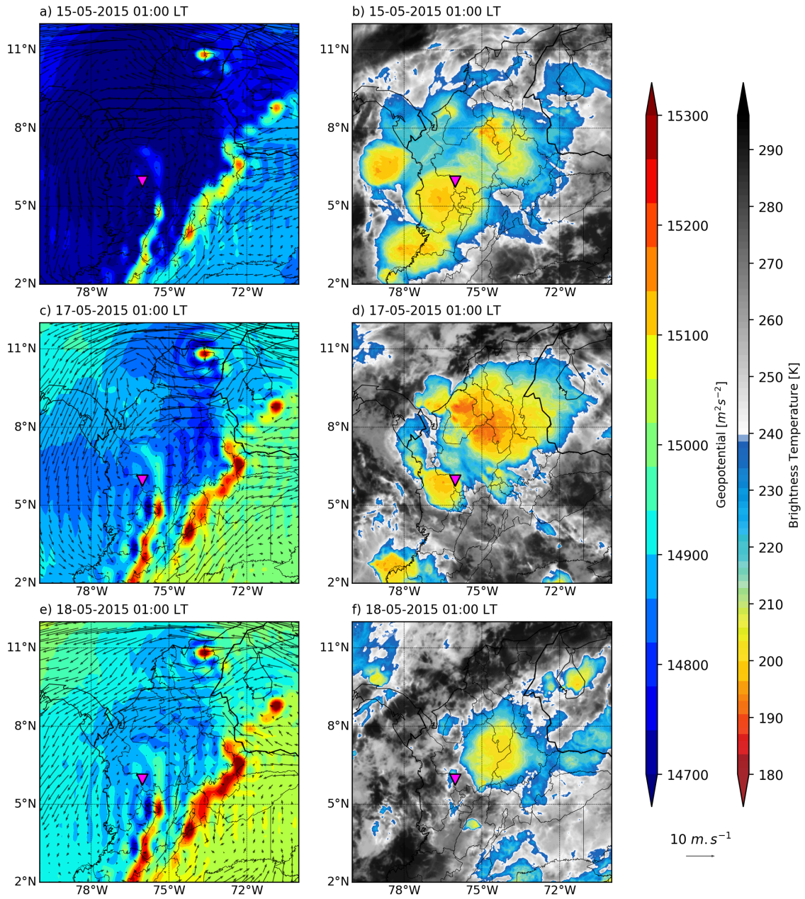
Figure 9. Panels a), c), and e) show the ERA Interim geopotential height at 700 hPa (filled contours) and horizontal wind (vectors) for May 15, 2015, May 17, 2015, and May 18, 2015, all at 01:00 LT, respectively. Panels b), d), and f) show the GOES-13 brightness temperature for the same times as in panels a), c), and e).
