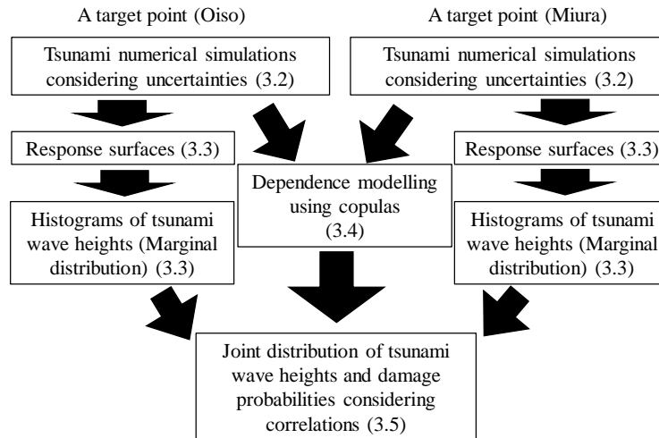
Figure 1: Flowchart of probabilistic tsunami hazard and risk assessment considering spatial correlation of tsunami wave height. Numbers in the parentheses indicate the section numbers described.
