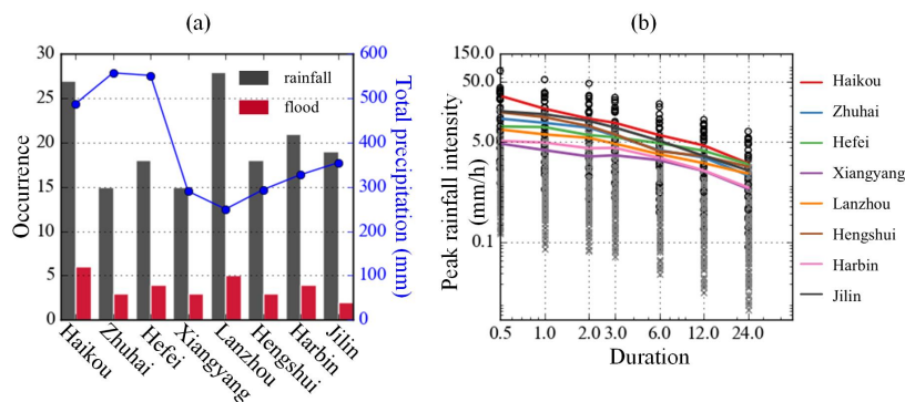
23 24 Figure 2. Total August precipitation and frequency of rainfall and city flooding events 25 (a). Variations in peak rainfall intensity (circles) and the flooding-triggering 26 precipitation threshold values (lines) that are derived from time windows ranging 27 from 0.5 to 24 hours (b). 28
