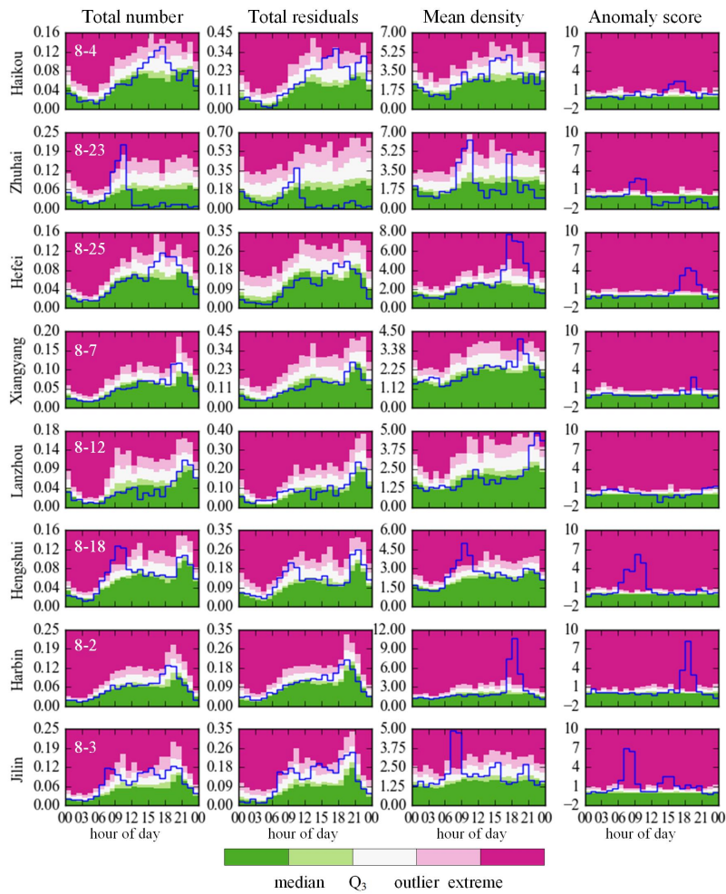
2 Figure 6. Intra-day variations in NLR, total residuals, mean density, and anomaly score 3 within 24 hours of a typical flooding event in each of the cities.
