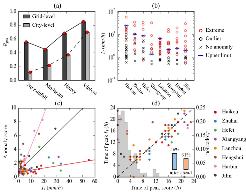
6 7 Figure 7. Correlation between peak rainfall intensity and anomaly score.
