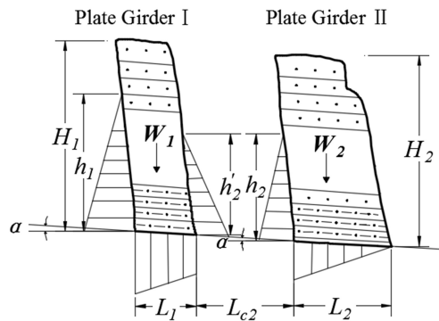
Fig. 9 Geomechanical model of two-stage plate-shaped sliding bodies
