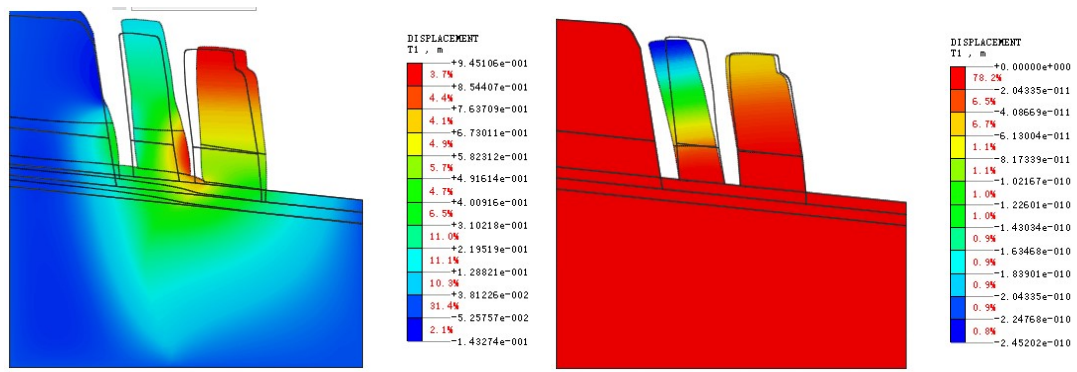
(c) The sliding bodies slide to the maximum state (d) Sliding bodies tilt backward when water level decreases Fig. 12 Example of finite element simulation and numerical calculation
