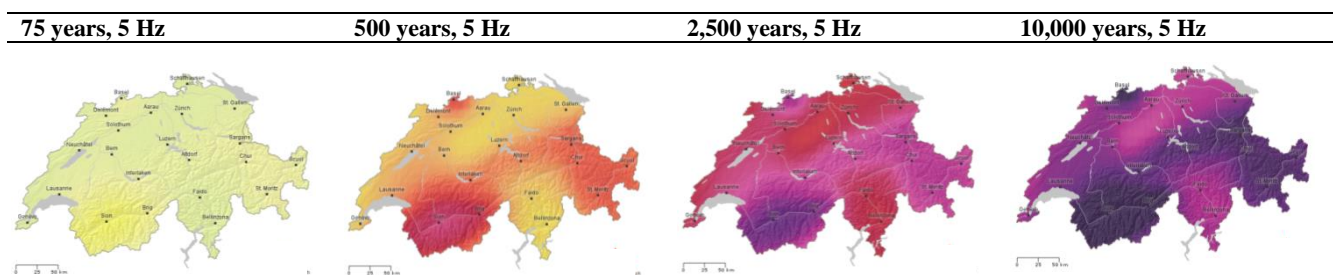
185 Fig. 4. Same color scale for hazard maps with different return periods (from left to right: 75 years, 500 years, 2,500 years, 10,000 years) (Swiss Seismological Service, 2018, www.seismo.ethz.ch/knowledge/seismic-hazard-switzerland/maps/hazard/ ).
