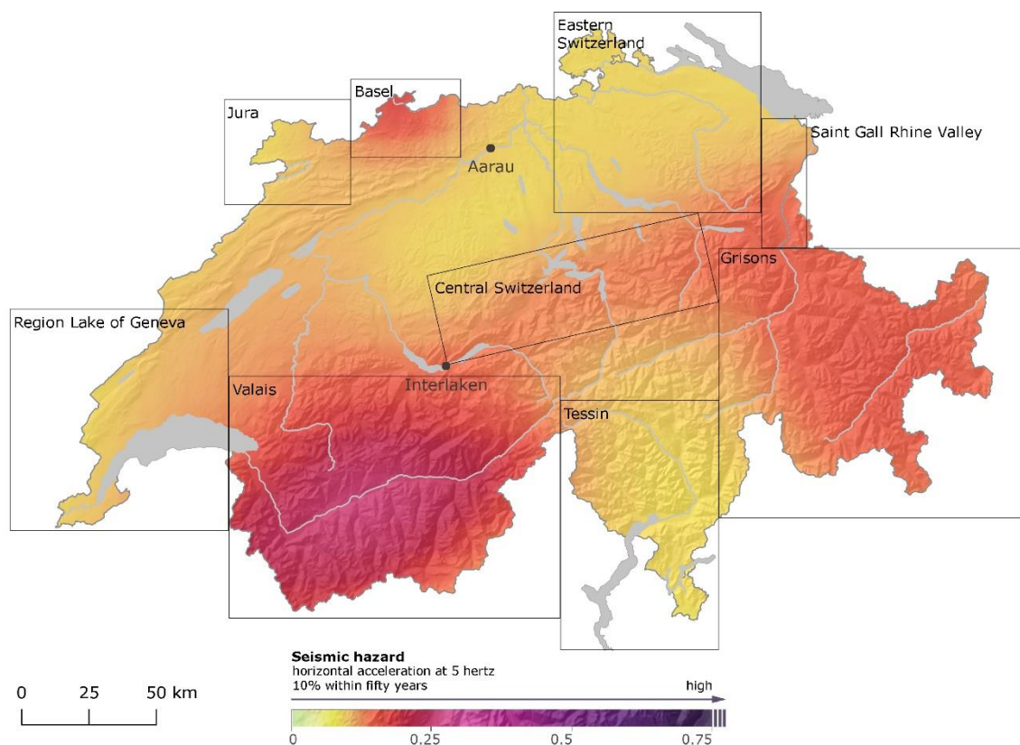
300 Fig. 6. Seismic hazard map displaying the probability of a horizontal acceleration at 5 Hertz to be experienced with 10 % within fifty years (475 years) on rocky subsoil and the areas in question (Swiss Seismological Service, 2018, www.seismo.ethz.ch/knowledge/seismic-hazard-switzerland/maps/hazard/ ). The map was shown to the participants without the frames highlighting the different areas.
