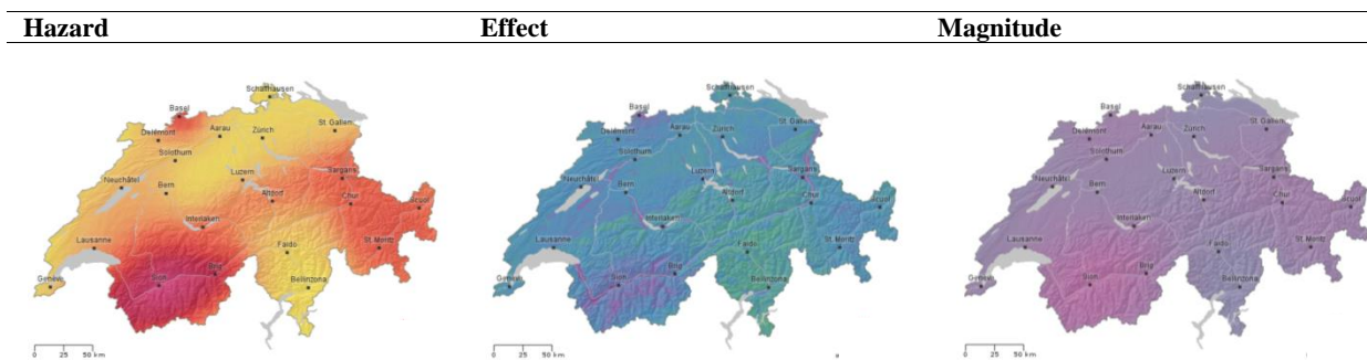
180 Fig. 3. Comparison of the color scales of the three map types offered for the release of the updated seismic hazard model: hazard map (in units of m/sec^2 ), effect map (in units of EMS Intensity) and magnitude map (in units of magnitude) (Swiss Seismological Service, 2018, www.seismo.ethz.ch/knowledge/seismic-hazard-switzerland/ ).
