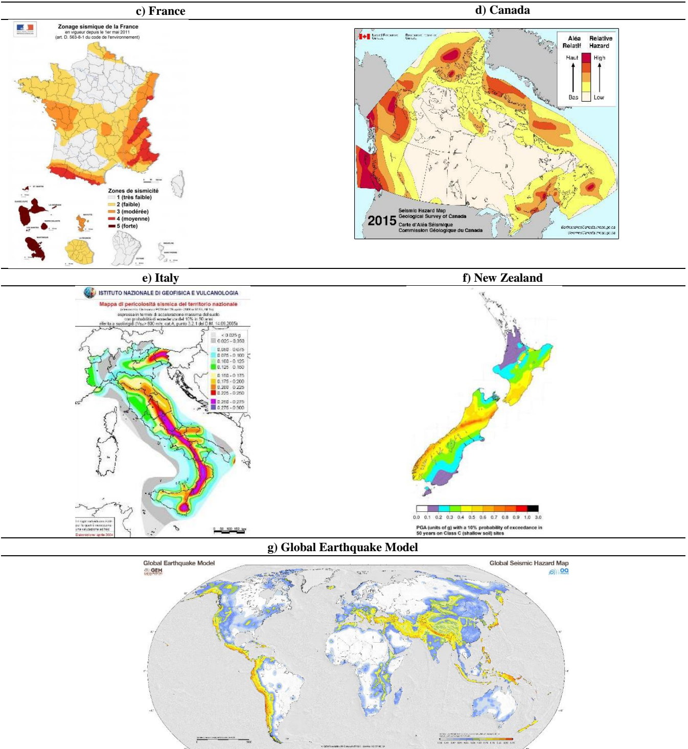
40 Fig. 1. Selection of national seismic hazard maps: a) Swiss seismic hazard map (Swiss Seismological Service, 2018, www.seismo.ethz.ch/knowledge/seismic-hazard-switzerland/ ) b) US seismic hazard map (United States Geological Survey, 2018, https://earthquake.usgs.gov/hazards/hazmaps/ ) c) Zonage sismique de la France (Bureau de recherches géologiques et minières, 2018,
