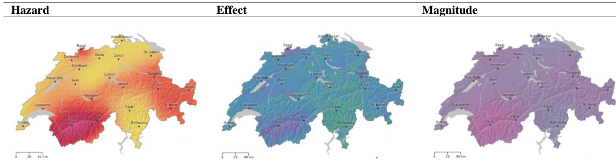
Fig. 3. Comparison of the color scales of the three map types offered for the release of the updated seismic hazard model: hazard map (in units of m/sec^2 ), effect map (in units of EMS Intensity) and magnitude map (in units of magnitude) (Swiss Seismological Service, 2018, www.seismo.ethz.ch/knowledge/seismic-hazard-switzerland/ ).
