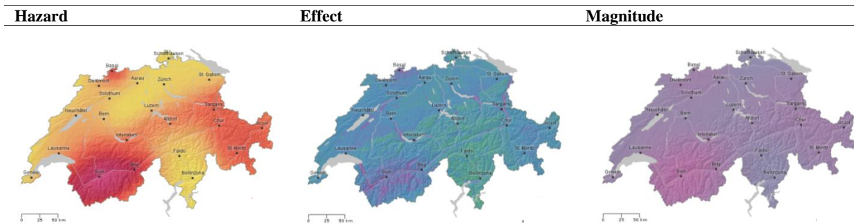
200 Fig. 3. Comparison of the color scales of the three map types offered for the release of the updated seismic hazard model: hazard map (in units of m/sec^2 ), effect map (in units of EMS Intensity) and magnitude map (in units of magnitude) (Swiss Seismological Service, 2018, www.seismo.ethz.ch/knowledge/seismic-hazard-switzerland/ ).
