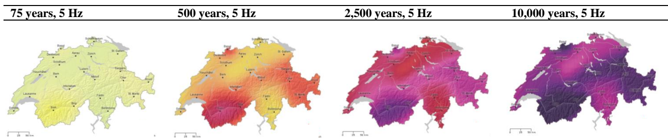
Fig. 4. Same color scale for hazard maps with different return periods (from left to right: 75 years, 500 years, 2,500 years, 10,000 years) (Swiss Seismological Service, 2018, www.seismo.ethz.ch/knowledge/seismic-hazard-switzerland/maps/hazard/ ).
