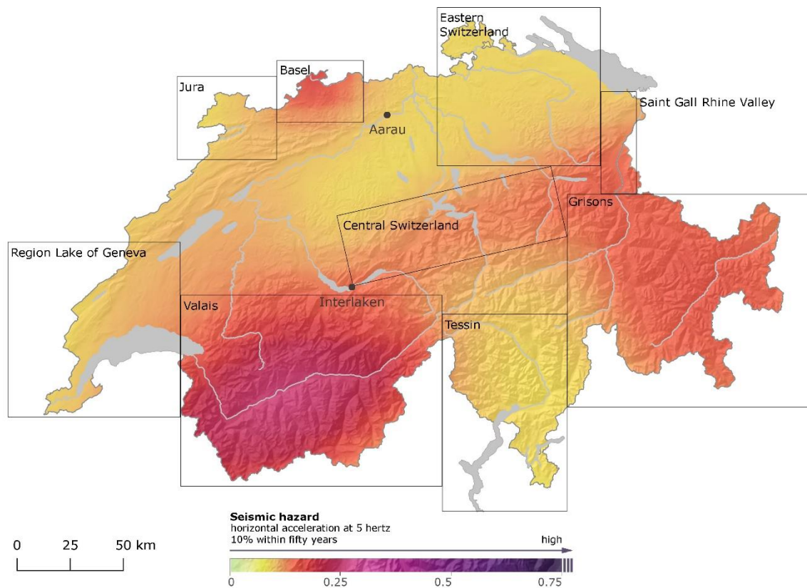
325 Fig. 6. Seismic hazard map displaying the probability of a horizontal acceleration at 5 Hertz to be experienced with 10 % within fifty years (475 years) on rocky subsoil and the areas in question (Swiss Seismological Service, 2018, www.seismo.ethz.ch/knowledge/seismic-hazard-switzerland/maps/hazard/ ). The map was shown to the participants without the frames highlighting the different areas.
