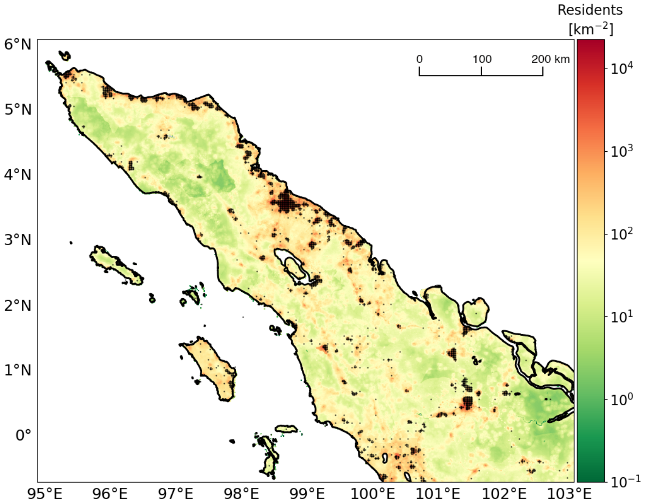
Figure 1. An example of a weighted grid used as an insurance density proxy for the location uncertainty framework. The map shows northern Sumatra. Color indicates population density (residents per \text{km}^2 ) as a proxy for insured exposure density. Black markers depict grid points of the weighted grid. The population data in this plot is based on a free dataset (Gaughan et al., 2015).
