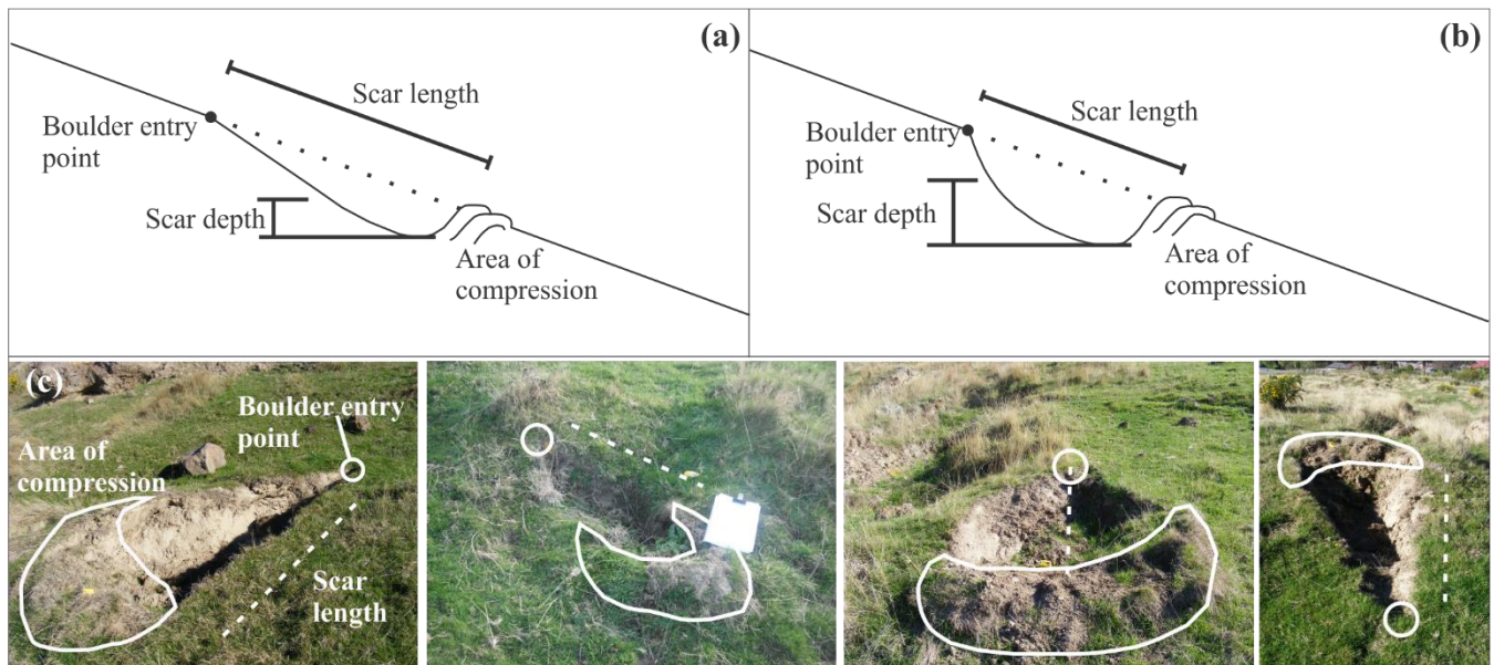
Figure 6. A. Schematic representation of impact scar morphology, where depth:length of the scar ratio is low, representing dry conditions, and high, representing wet conditions (B). C. Images of impact scars from Rapaki Bay showing typical scar morphology from four different boulders.
