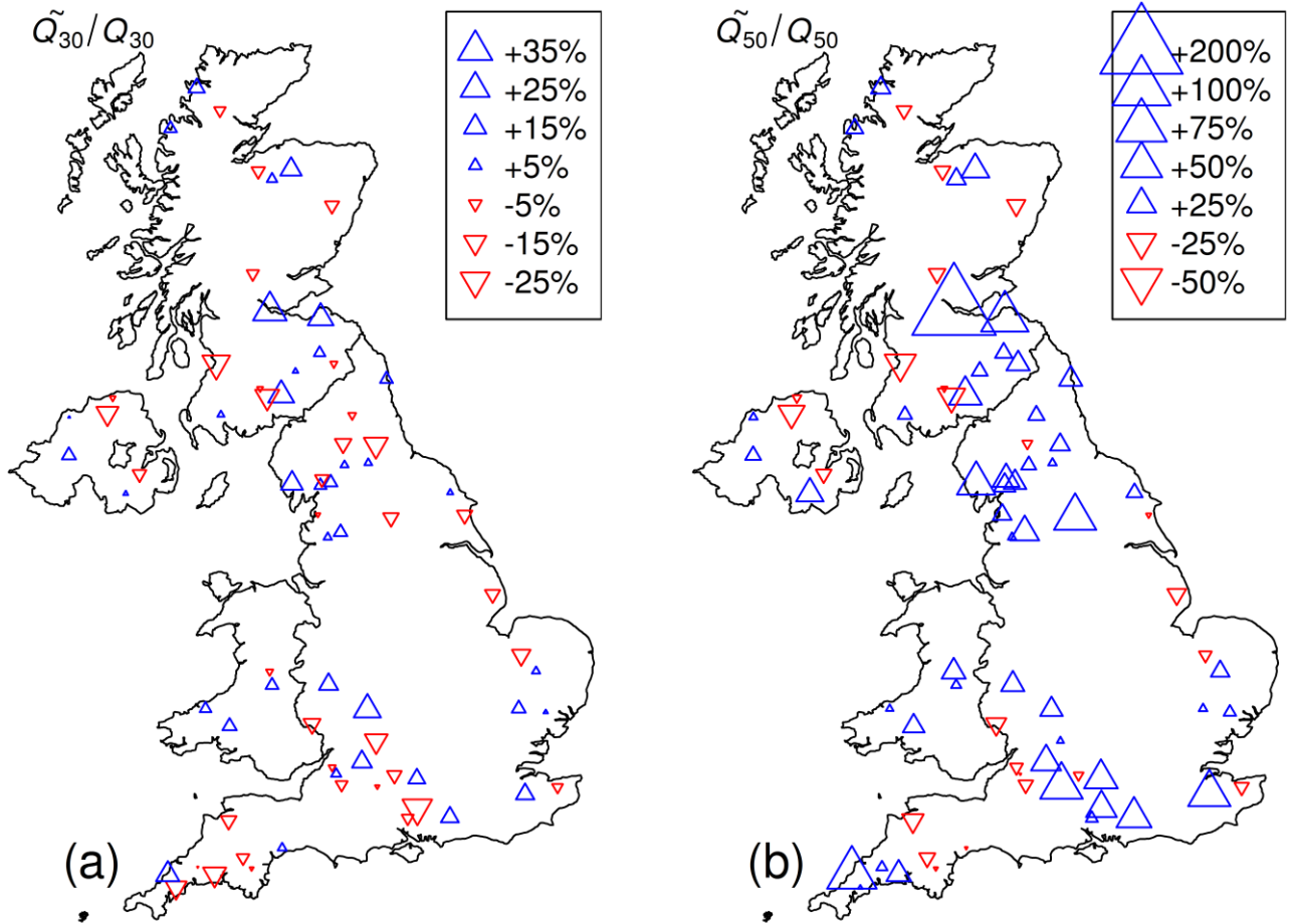
Figure 9: Percentage change of long-return period flood magnitudes \left(\frac{\bar{Q}_T}{Q_T} - 1\right) \times 100\% computed under assumptions of stationarity ( Q_T ) and non-stationary probability of exceedance ( \bar{Q}_T ). Shown for the 30-year event (a) and 50-year event (b).
