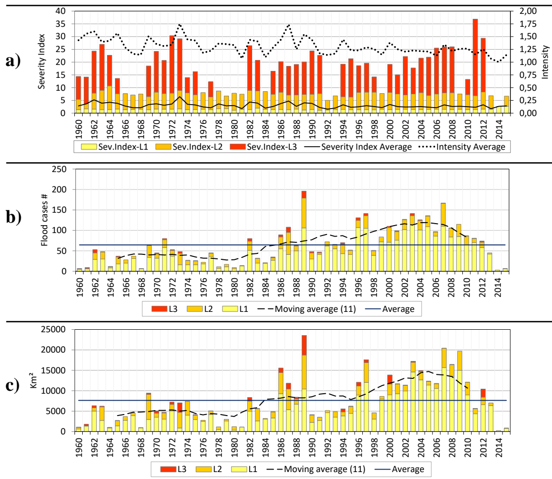
Figure 7: Temporal variability of the intensity, severity and spatial impact of flood cases in the SMC.
