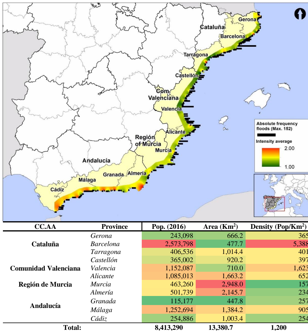
Figure 3: Intensity average and total flood cases by municipality and Spanish Mediterranean coastal municipalities, spatial summary. The map shows in different colours the average intensity of flood cases in each municipality, and the black bars represent the total number of flood cases in each municipality. 5 The table reports the total population, the total area and the population density by province. The different colours represent how the values deviate above (from yellow to red colours) or below (from yellow to green colours) from the 50th percentile within the mean values of the variables (Pop., Area and Density). Source: INE, 2018.
