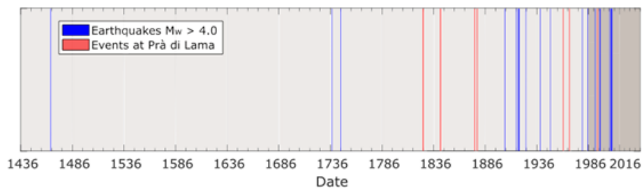
Fig. 3. Figure 3 - Historical record of the events occurred at Prà di Lama (red lines) and earthquakes occurred in the Garfagnana graben (blue lines). The historical seismicity record has been obtained from
